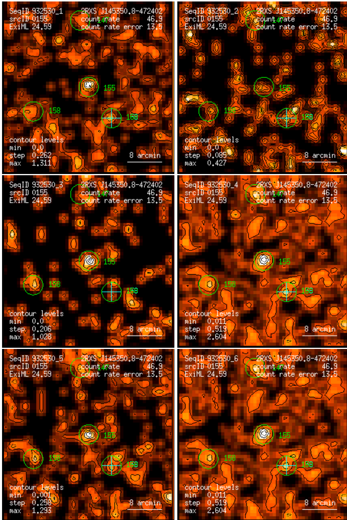
Figure 155: RASS 932530: detection 0155: band rate images, Gaussian filter: (1) PSPC channels 11 – 41, (2) 52 – 90, (3) 91 – 201, (4) 11 – 235, (5) 52 – 201, (6) 11 – 201. Broad band rates in counts/ks. Band rate contour levels in counts/ks/arcmin 2 .
