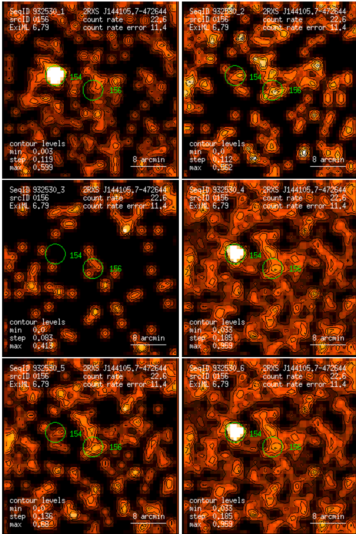
Figure 156: RASS 932530: detection 0156: band rate images, Gaussian filter: (1) PSPC channels 11 – 41, (2) 52 – 90, (3) 91 – 201, (4) 11 – 235, (5) 52 – 201, (6) 11 – 201. Broad band rates in counts/ks. Band rate contour levels in counts/ks/arcmin 2 .
