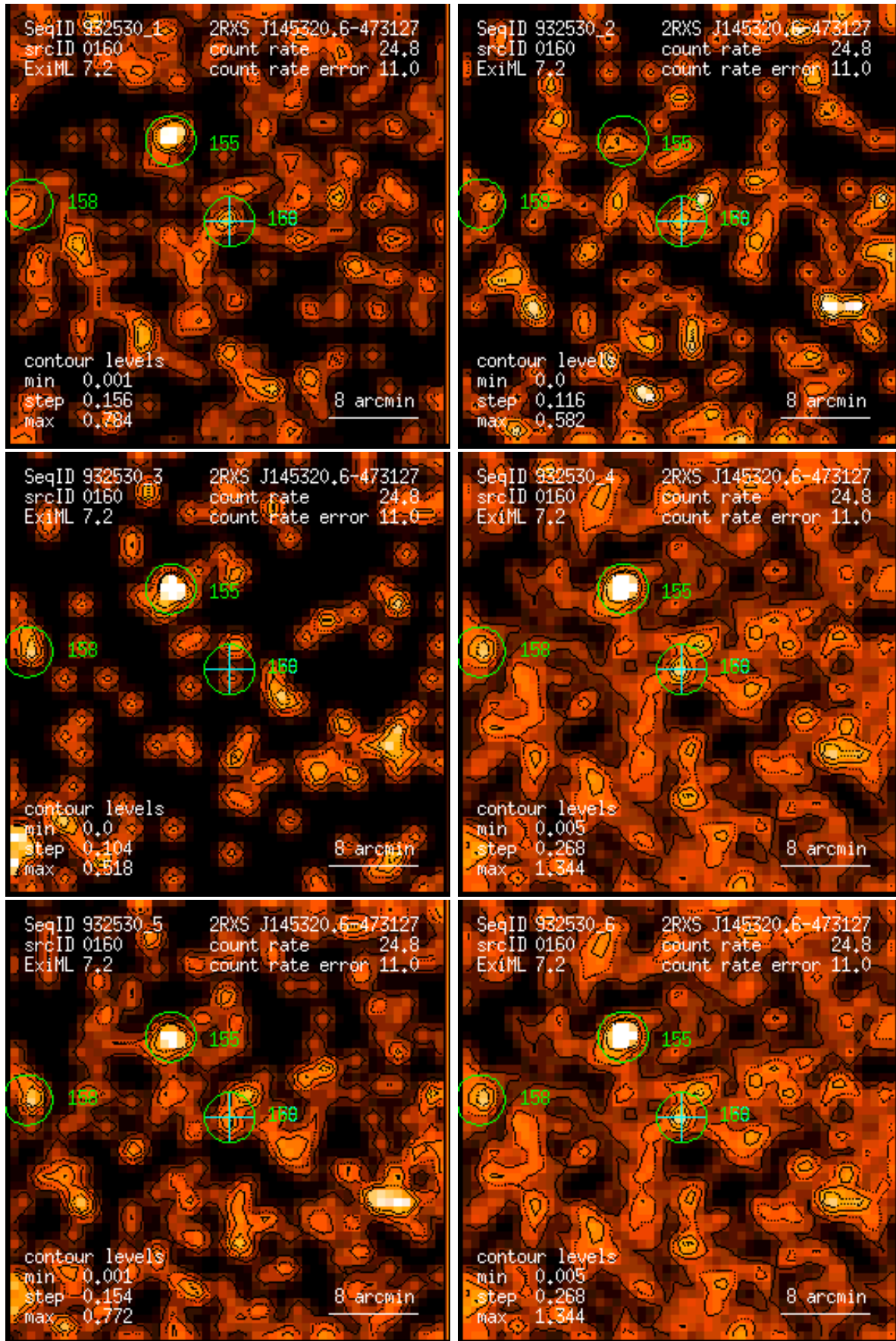
Figure 160: RASS 932530: detection 0160: band rate images, Gaussian filter: (1) PSPC channels 11 – 41, (2) 52 – 90, (3) 91 – 201, (4) 11 – 235, (5) 52 – 201, (6) 11 – 201. Broad band rates in counts/ks. Band rate contour levels in counts/ks/arcmin 2 .
