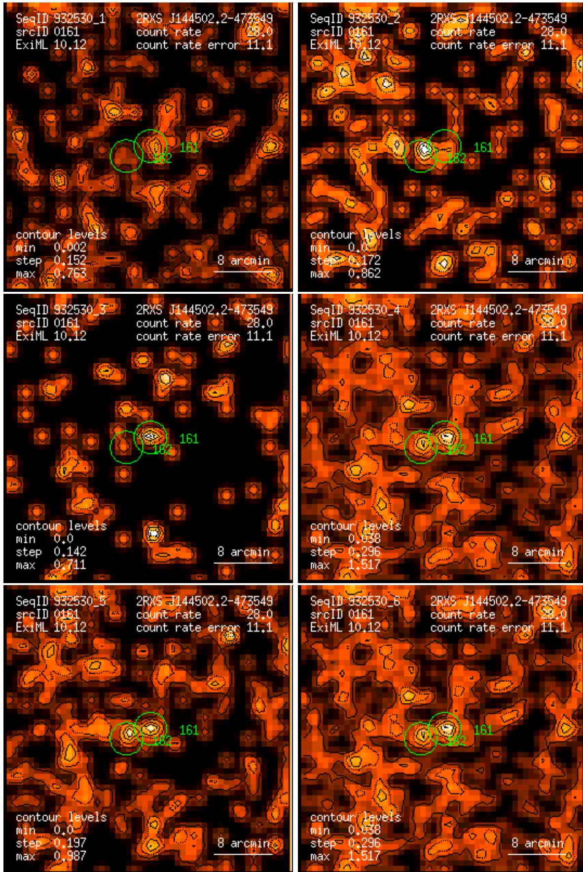
Figure 161: RASS 932530: detection 0161: band rate images, Gaussian filter: (1) PSPC channels 11 – 41, (2) 52 – 90, (3) 91 – 201, (4) 11 – 235, (5) 52 – 201, (6) 11 – 201. Broad band rates in counts/ks. Band rate contour levels in counts/ks/arcmin 2 .
