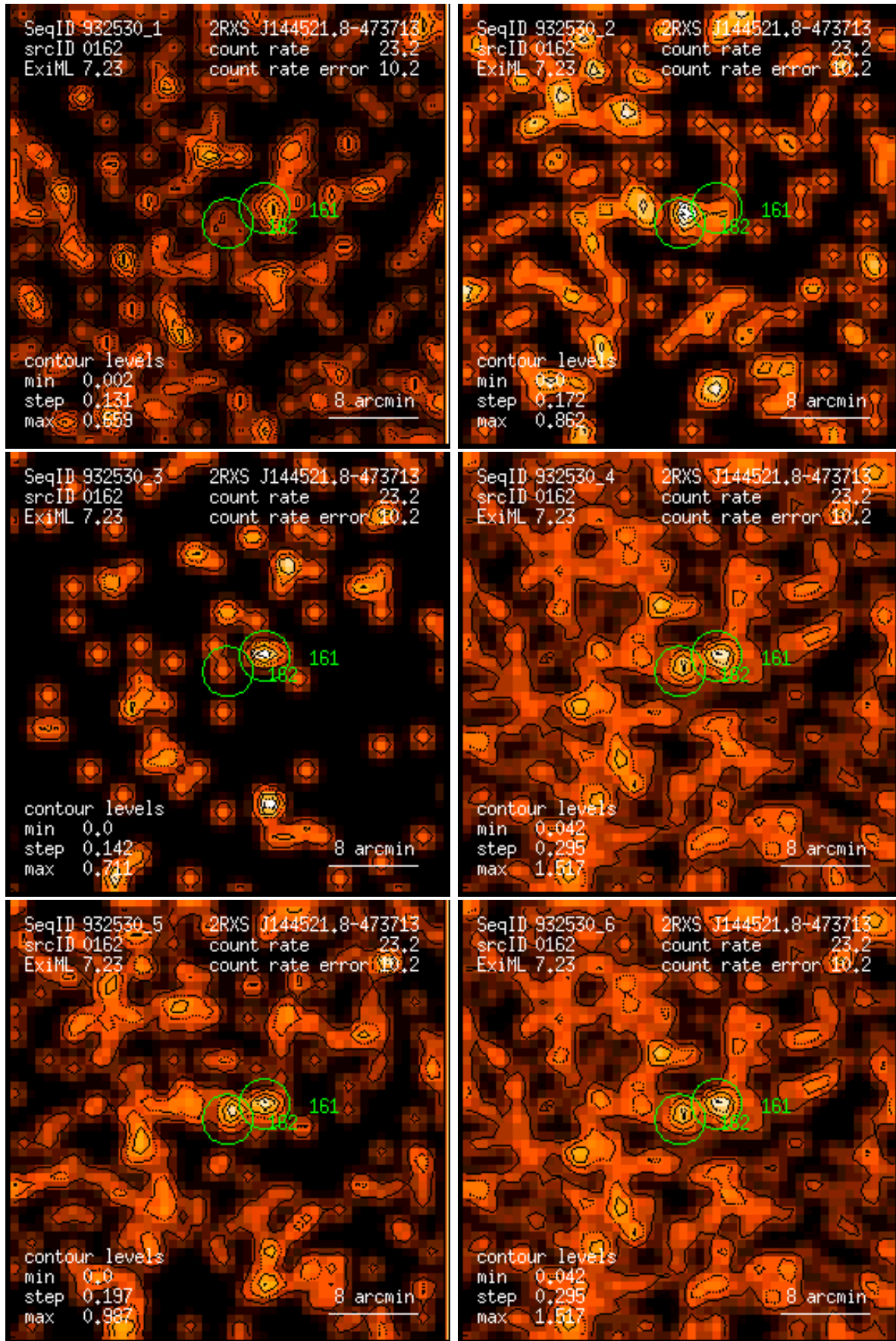
Figure 162: RASS 932530: detection 0162: band rate images, Gaussian filter: (1) PSPC channels 11 – 41, (2) 52 – 90, (3) 91 – 201, (4) 11 – 235, (5) 52 – 201, (6) 11 – 201. Broad band rates in counts/ks. Band rate contour levels in counts/ks/arcmin 2 .
