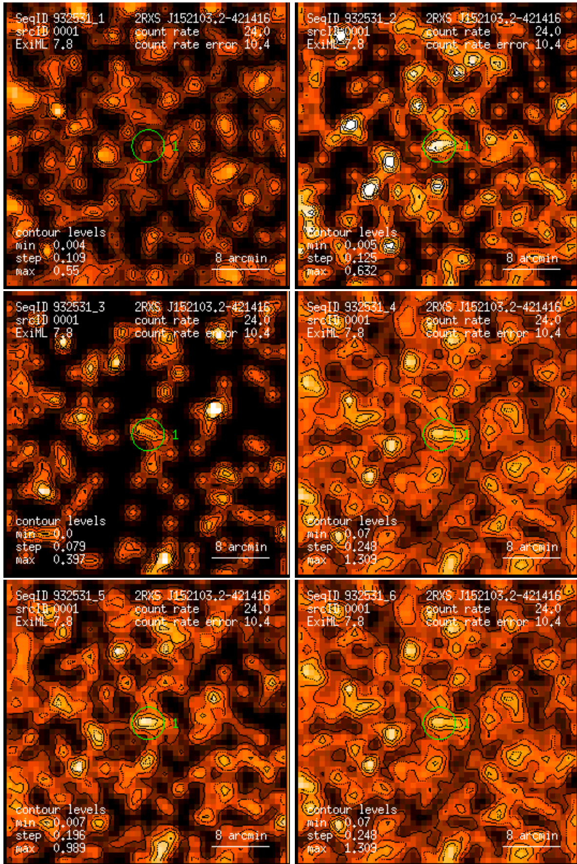
Figure 1: RASS 932531: detection 0001: band rate images, Gaussian filter: (1) PSPC channels 11 – 41, (2) 52 – 90, (3) 91 – 201, (4) 11 – 235, (5) 52 – 201, (6) 11 – 201. Broad band rates in counts/ks. Band rate contour levels in counts/ks/arcmin 2 .
