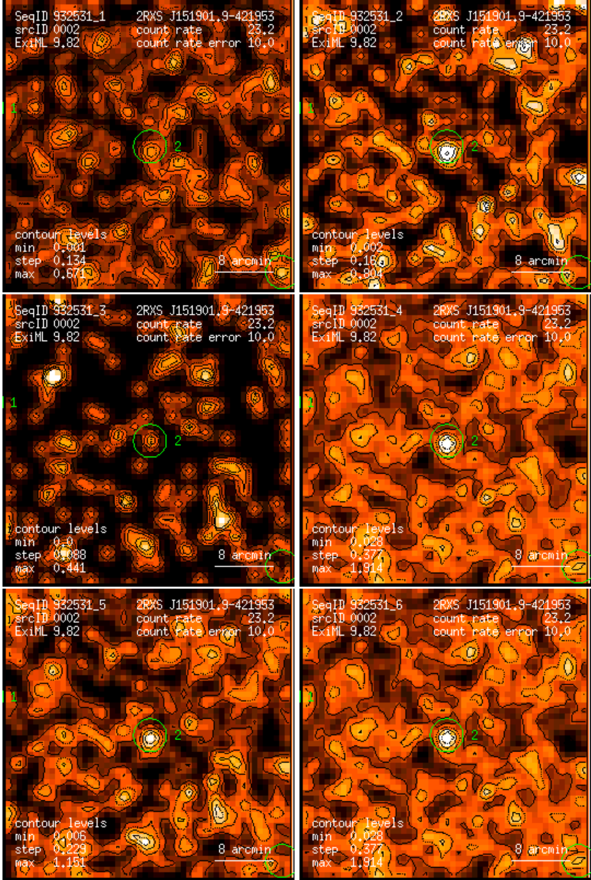
Figure 2: RASS 932531: detection 0002: band rate images, Gaussian filter: (1) PSPC channels 11 – 41, (2) 52 – 90, (3) 91 – 201, (4) 11 – 235, (5) 52 – 201, (6) 11 – 201. Broad band rates in counts/ks. Band rate contour levels in counts/ks/arcmin 2 .
