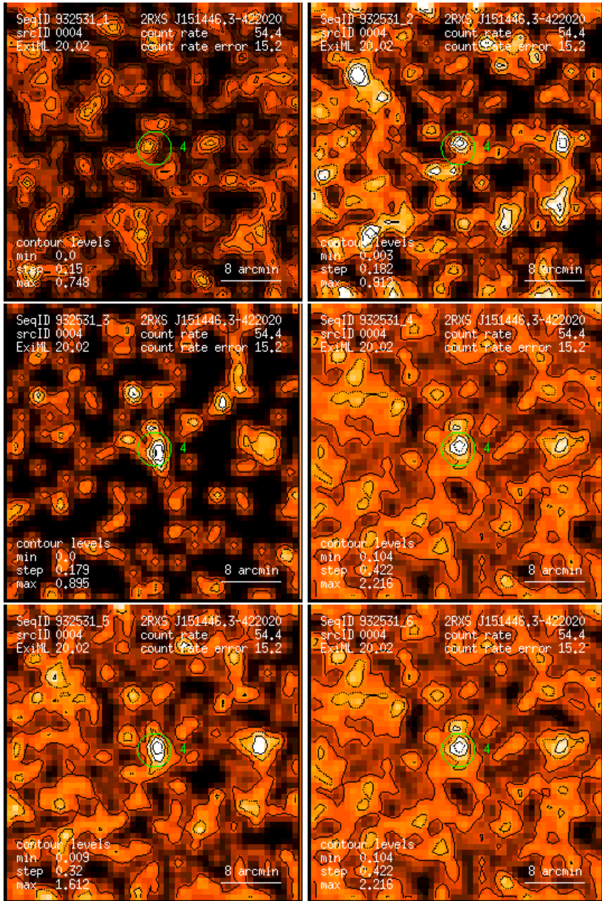
Figure 4: RASS 932531: detection 0004: band rate images, Gaussian filter: (1) PSPC channels 11 – 41, (2) 52 – 90, (3) 91 – 201, (4) 11 – 235, (5) 52 – 201, (6) 11 – 201. Broad band rates in counts/ks. Band rate contour levels in counts/ks/arcmin 2 .
