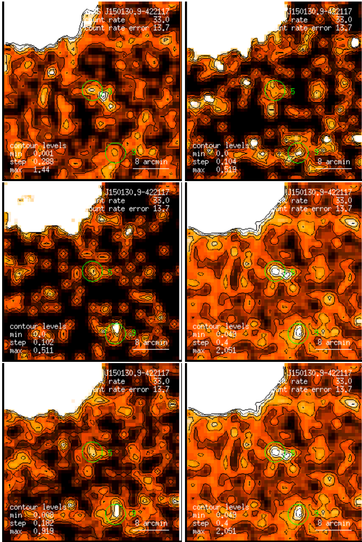
Figure 5: RASS 932531: detection 0005: band rate images, Gaussian filter: (1) PSPC channels 11 – 41, (2) 52 – 90, (3) 91 – 201, (4) 11 – 235, (5) 52 – 201, (6) 11 – 201. Broad band rates in counts/ks. Band rate contour levels in counts/ks/arcmin 2 .
