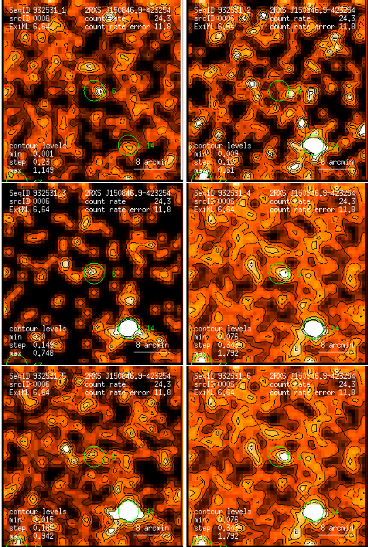
Figure 6: RASS 932531: detection 0006: band rate images, Gaussian filter: (1) PSPC channels 11 – 41, (2) 52 – 90, (3) 91 – 201, (4) 11 – 235, (5) 52 – 201, (6) 11 – 201. Broad band rates in counts/ks. Band rate contour levels in counts/ks/arcmin 2 .
