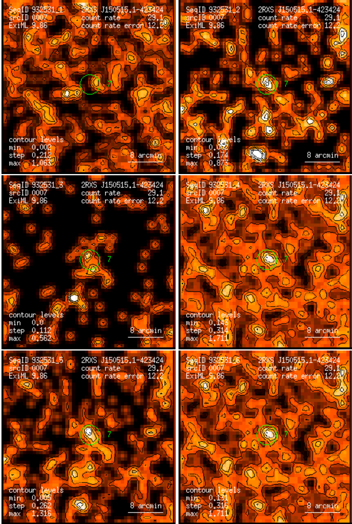
Figure 7: RASS 932531: detection 0007: band rate images, Gaussian filter: (1) PSPC channels 11 – 41, (2) 52 – 90, (3) 91 – 201, (4) 11 – 235, (5) 52 – 201, (6) 11 – 201. Broad band rates in counts/ks. Band rate contour levels in counts/ks/arcmin 2 .
