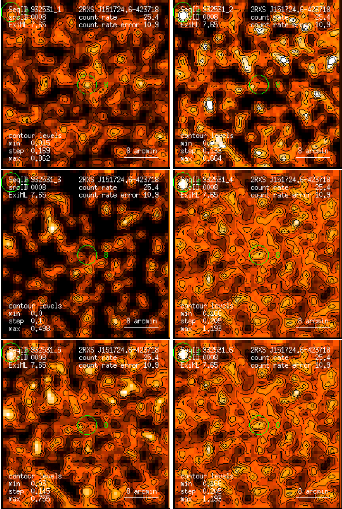
Figure 8: RASS 932531: detection 0008: band rate images, Gaussian filter: (1) PSPC channels 11 – 41, (2) 52 – 90, (3) 91 – 201, (4) 11 – 235, (5) 52 – 201, (6) 11 – 201. Broad band rates in counts/ks. Band rate contour levels in counts/ks/arcmin 2 .
