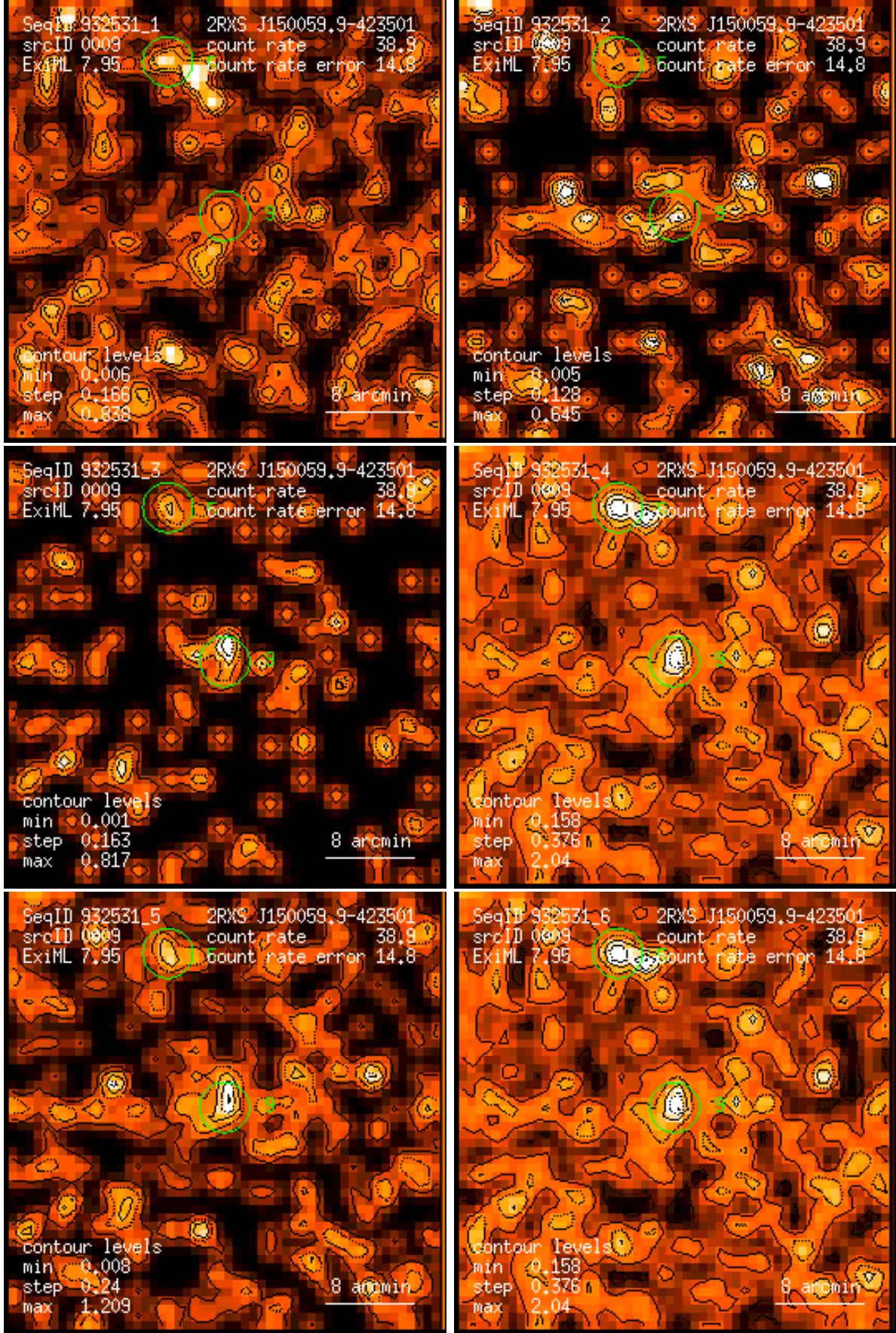
Figure 9: RASS 932531: detection 0009: band rate images, Gaussian filter: (1) PSPC channels 11 – 41, (2) 52 – 90, (3) 91 – 201, (4) 11 – 235, (5) 52 – 201, (6) 11 – 201. Broad band rates in counts/ks. Band rate contour levels in counts/ks/arcmin 2 .
