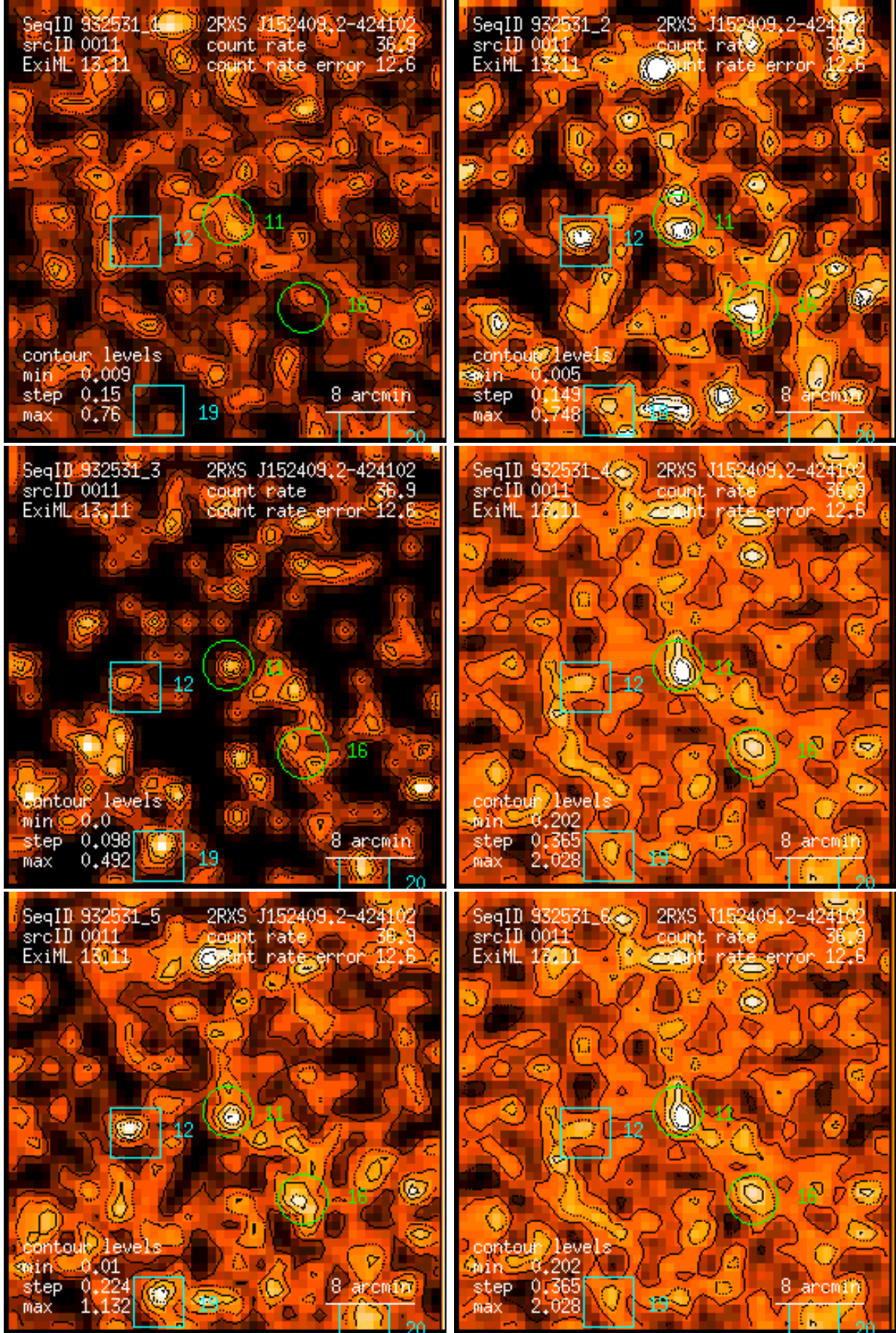
Figure 11: RASS 932531: detection 0011: band rate images, Gaussian filter: (1) PSPC channels 11 – 41, (2) 52 – 90, (3) 91 – 201, (4) 11 – 235, (5) 52 – 201, (6) 11 – 201. Broad band rates in counts/ks. Band rate contour levels in counts/ks/arcmin 2 .
