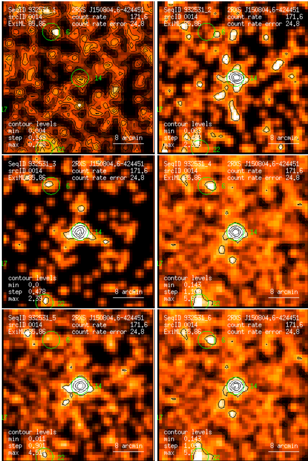
Figure 14: RASS 932531: detection 0014: band rate images, Gaussian filter: (1) PSPC channels 11 – 41, (2) 52 – 90, (3) 91 – 201, (4) 11 – 235, (5) 52 – 201, (6) 11 – 201. Broad band rates in counts/ks. Band rate contour levels in counts/ks/arcmin 2 .
