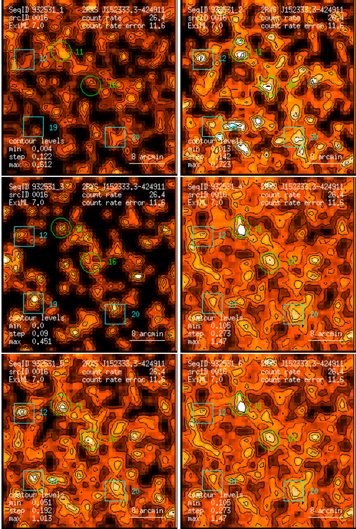
Figure 16: RASS 932531: detection 0016: band rate images, Gaussian filter: (1) PSPC channels 11 – 41, (2) 52 – 90, (3) 91 – 201, (4) 11 – 235, (5) 52 – 201, (6) 11 – 201. Broad band rates in counts/ks. Band rate contour levels in counts/ks/arcmin 2 .
