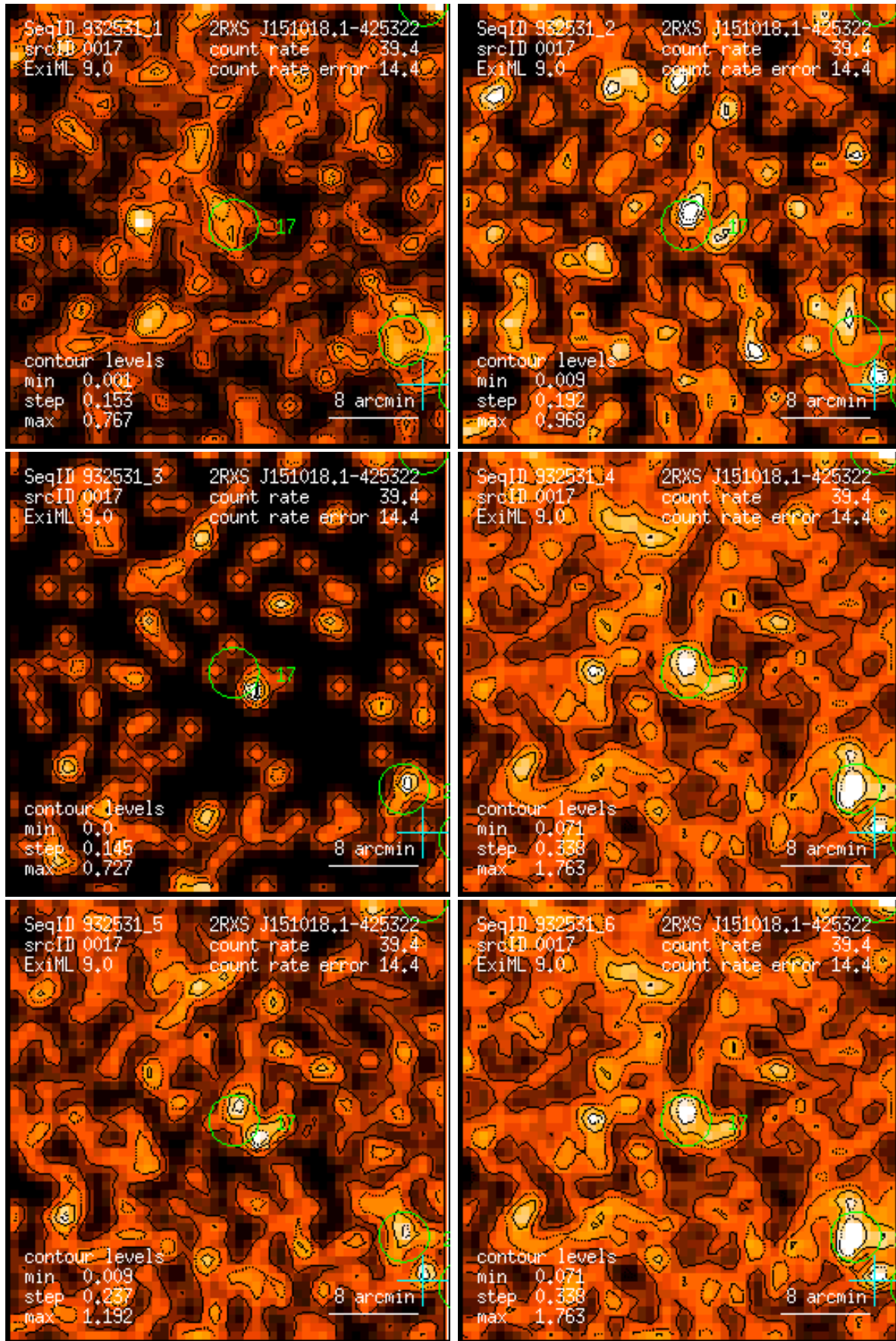
Figure 17: RASS 932531: detection 0017: band rate images, Gaussian filter: (1) PSPC channels 11 – 41, (2) 52 – 90, (3) 91 – 201, (4) 11 – 235, (5) 52 – 201, (6) 11 – 201. Broad band rates in counts/ks. Band rate contour levels in counts/ks/arcmin 2 .
