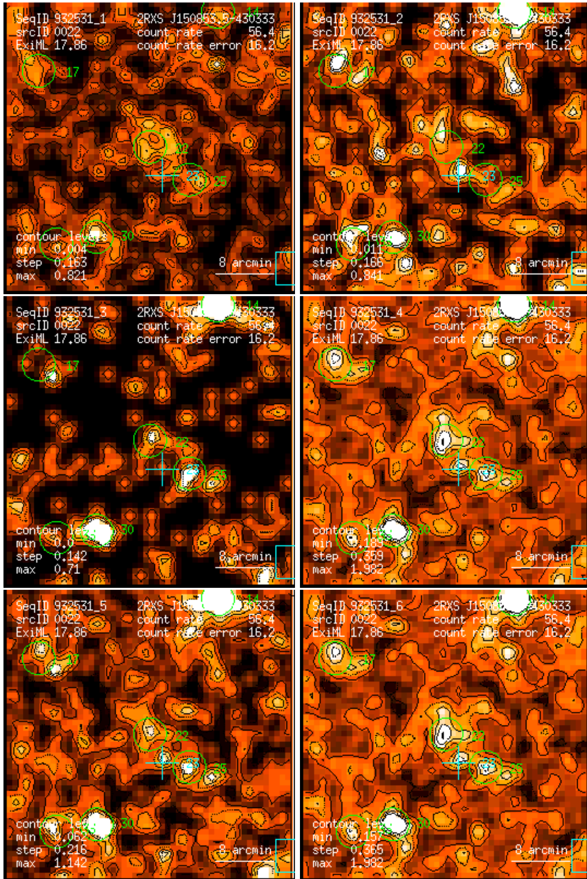
Figure 22: RASS 932531: detection 0022: band rate images, Gaussian filter: (1) PSPC channels 11 – 41, (2) 52 – 90, (3) 91 – 201, (4) 11 – 235, (5) 52 – 201, (6) 11 – 201. Broad band rates in counts/ks. Band rate contour levels in counts/ks/arcmin 2 .
