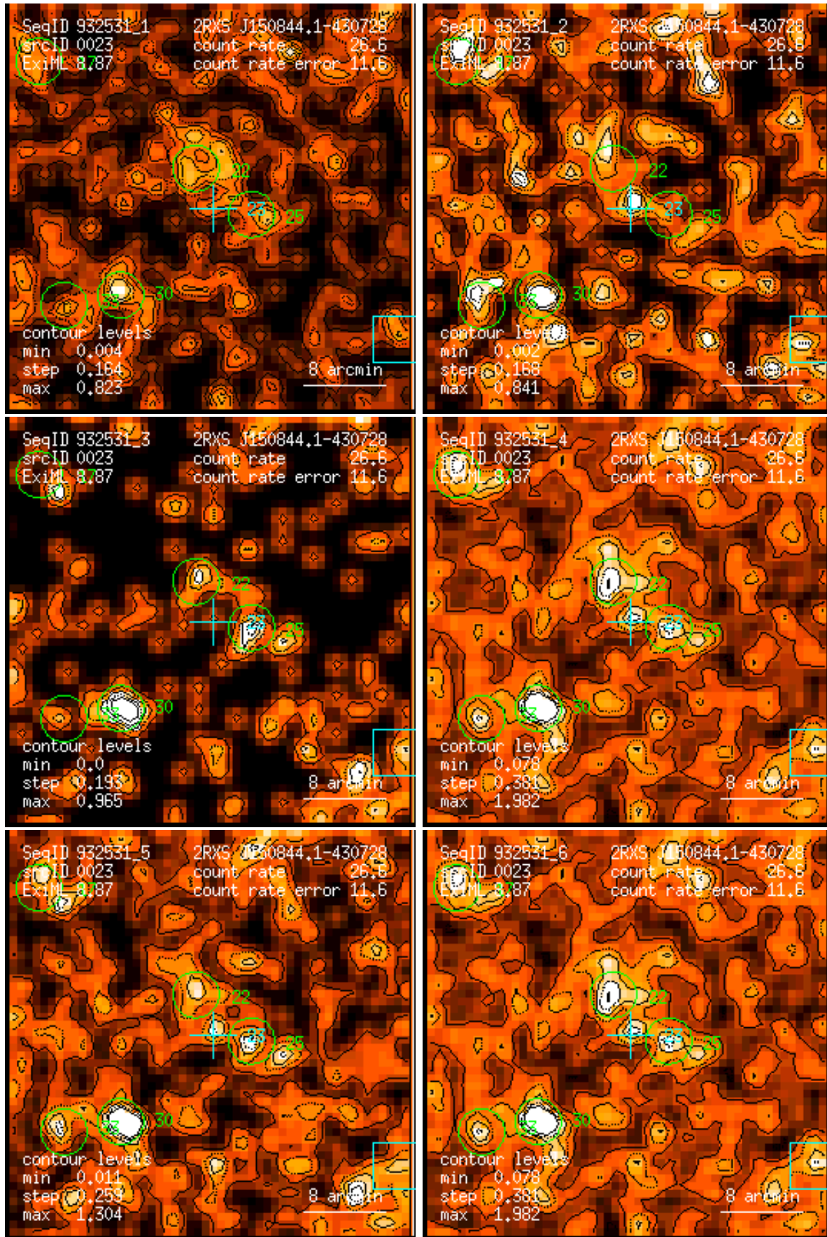
Figure 23: RASS 932531: detection 0023: band rate images, Gaussian filter: (1) PSPC channels 11 – 41, (2) 52 – 90, (3) 91 – 201, (4) 11 – 235, (5) 52 – 201, (6) 11 – 201. Broad band rates in counts/ks. Band rate contour levels in counts/ks/arcmin 2 .
