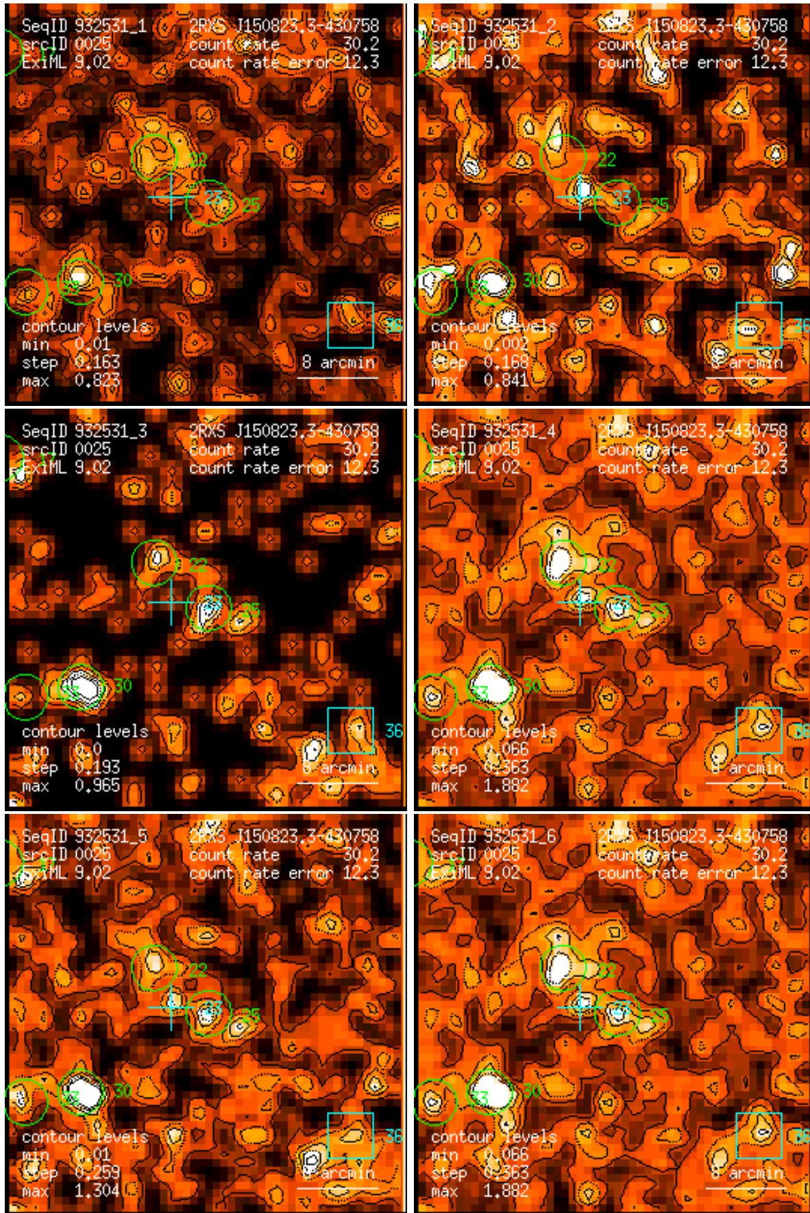
Figure 25: RASS 932531: detection 0025: band rate images, Gaussian filter: (1) PSPC channels 11 – 41, (2) 52 – 90, (3) 91 – 201, (4) 11 – 235, (5) 52 – 201, (6) 11 – 201. Broad band rates in counts/ks. Band rate contour levels in counts/ks/arcmin 2 .
