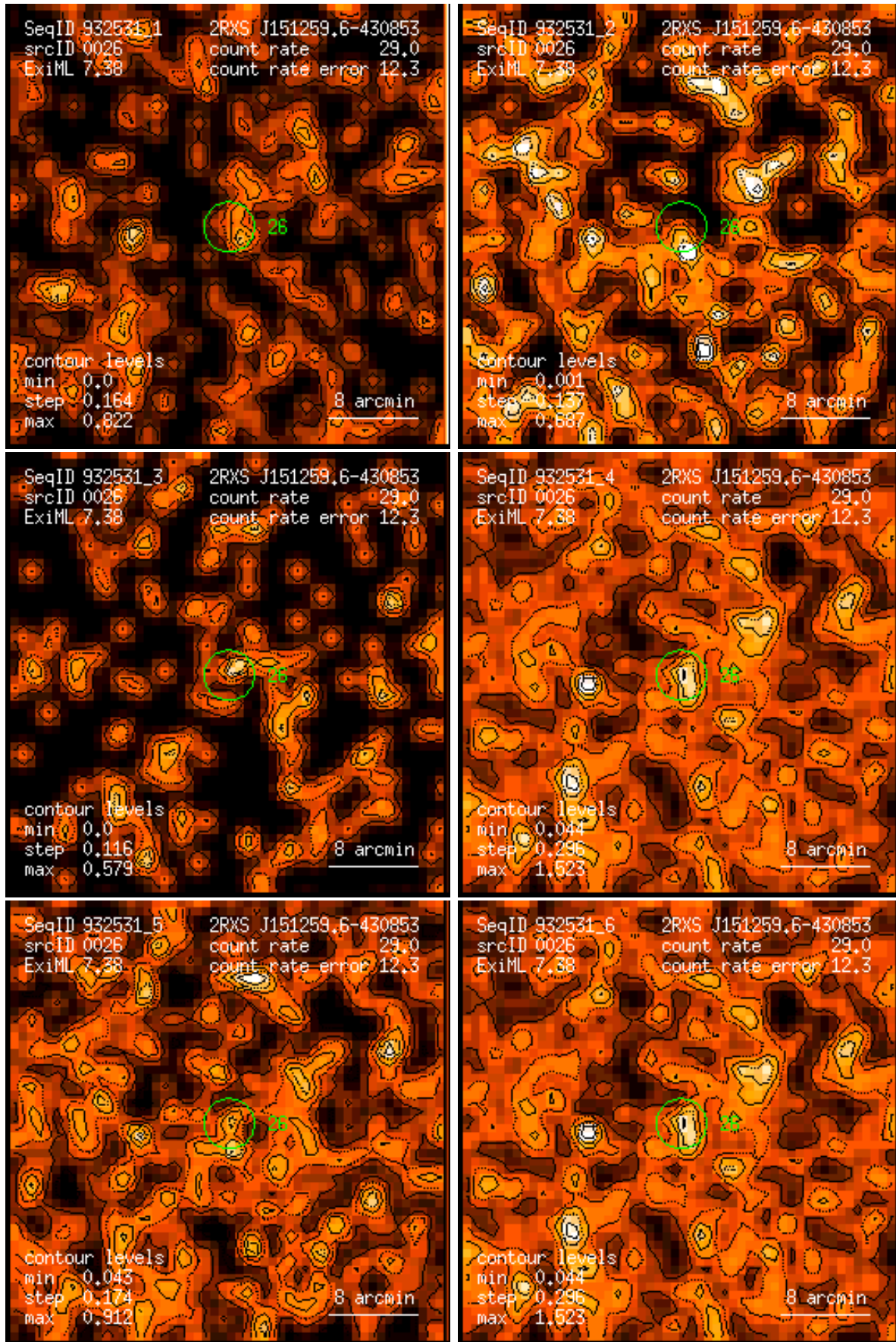
Figure 26: RASS 932531: detection 0026: band rate images, Gaussian filter: (1) PSPC channels 11 – 41, (2) 52 – 90, (3) 91 – 201, (4) 11 – 235, (5) 52 – 201, (6) 11 – 201. Broad band rates in counts/ks. Band rate contour levels in counts/ks/arcmin 2 .
