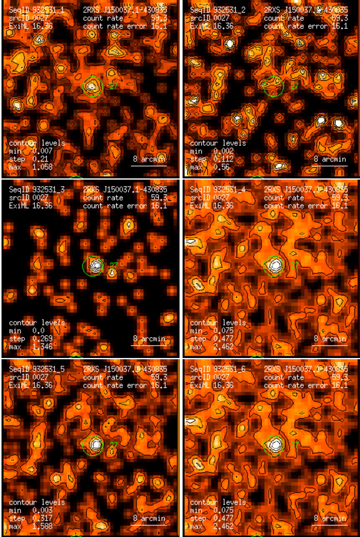
Figure 27: RASS 932531: detection 0027: band rate images, Gaussian filter: (1) PSPC channels 11 – 41, (2) 52 – 90, (3) 91 – 201, (4) 11 – 235, (5) 52 – 201, (6) 11 – 201. Broad band rates in counts/ks. Band rate contour levels in counts/ks/arcmin 2 .
