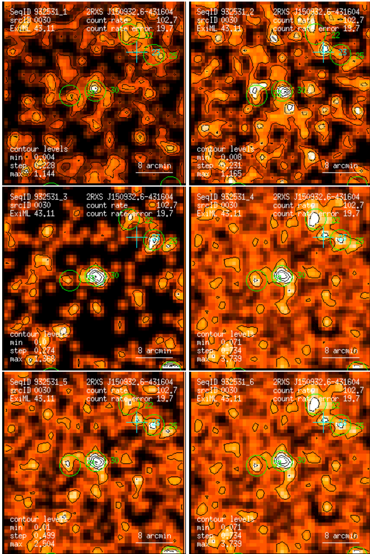
Figure 30: RASS 932531: detection 0030: band rate images, Gaussian filter: (1) PSPC channels 11 – 41, (2) 52 – 90, (3) 91 – 201, (4) 11 – 235, (5) 52 – 201, (6) 11 – 201. Broad band rates in counts/ks. Band rate contour levels in counts/ks/arcmin 2 .
