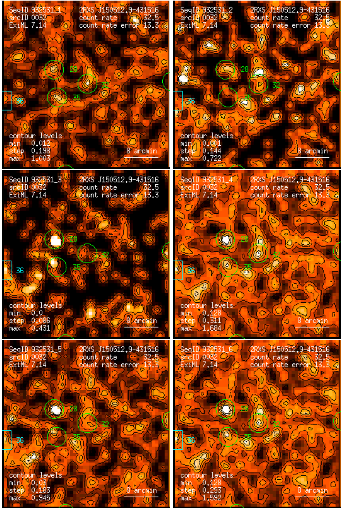
Figure 32: RASS 932531: detection 0032: band rate images, Gaussian filter: (1) PSPC channels 11 – 41, (2) 52 – 90, (3) 91 – 201, (4) 11 – 235, (5) 52 – 201, (6) 11 – 201. Broad band rates in counts/ks. Band rate contour levels in counts/ks/arcmin 2 .
