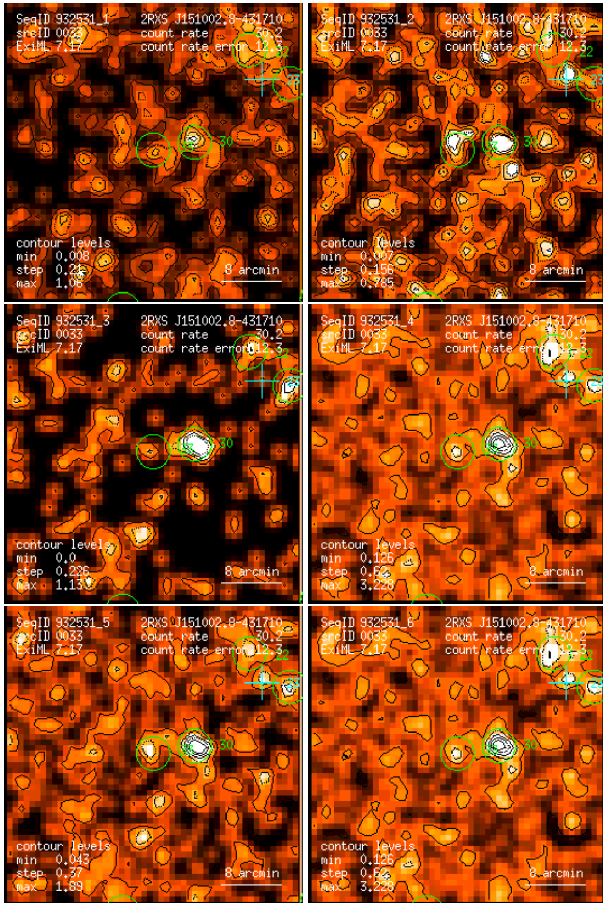
Figure 33: RASS 932531: detection 0033: band rate images, Gaussian filter: (1) PSPC channels 11 – 41, (2) 52 – 90, (3) 91 – 201, (4) 11 – 235, (5) 52 – 201, (6) 11 – 201. Broad band rates in counts/ks. Band rate contour levels in counts/ks/arcmin 2 .
