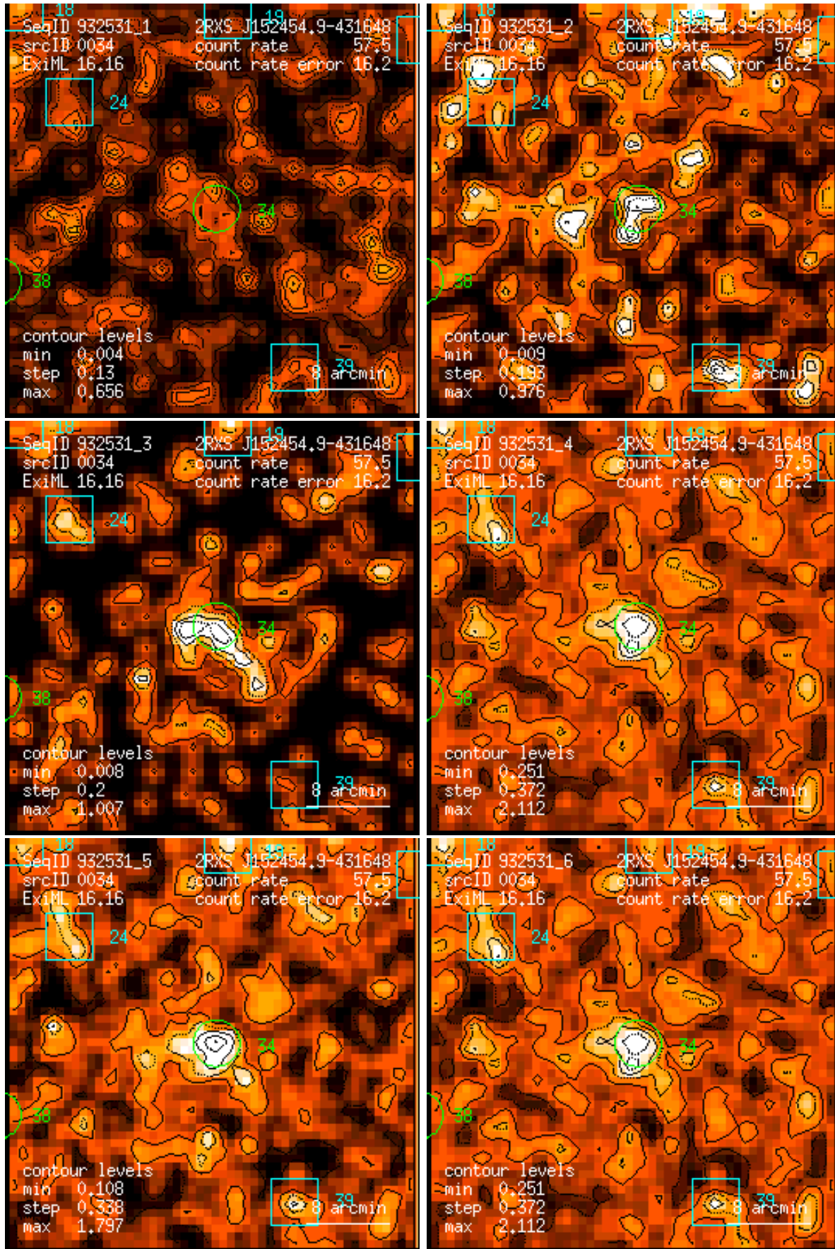
Figure 34: RASS 932531: detection 0034: band rate images, Gaussian filter: (1) PSPC channels 11 – 41, (2) 52 – 90, (3) 91 – 201, (4) 11 – 235, (5) 52 – 201, (6) 11 – 201. Broad band rates in counts/ks. Band rate contour levels in counts/ks/arcmin 2 .
