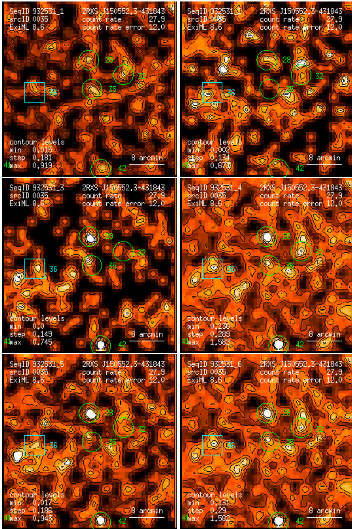
Figure 35: RASS 932531: detection 0035: band rate images, Gaussian filter: (1) PSPC channels 11 – 41, (2) 52 – 90, (3) 91 – 201, (4) 11 – 235, (5) 52 – 201, (6) 11 – 201. Broad band rates in counts/ks. Band rate contour levels in counts/ks/arcmin 2 .
