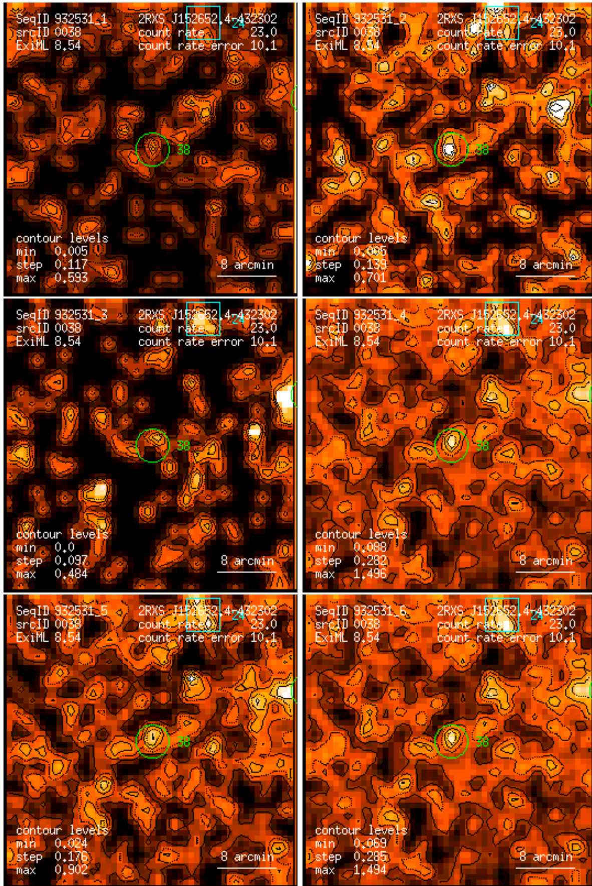
Figure 38: RASS 932531: detection 0038: band rate images, Gaussian filter: (1) PSPC channels 11 – 41, (2) 52 – 90, (3) 91 – 201, (4) 11 – 235, (5) 52 – 201, (6) 11 – 201. Broad band rates in counts/ks. Band rate contour levels in counts/ks/arcmin 2 .
