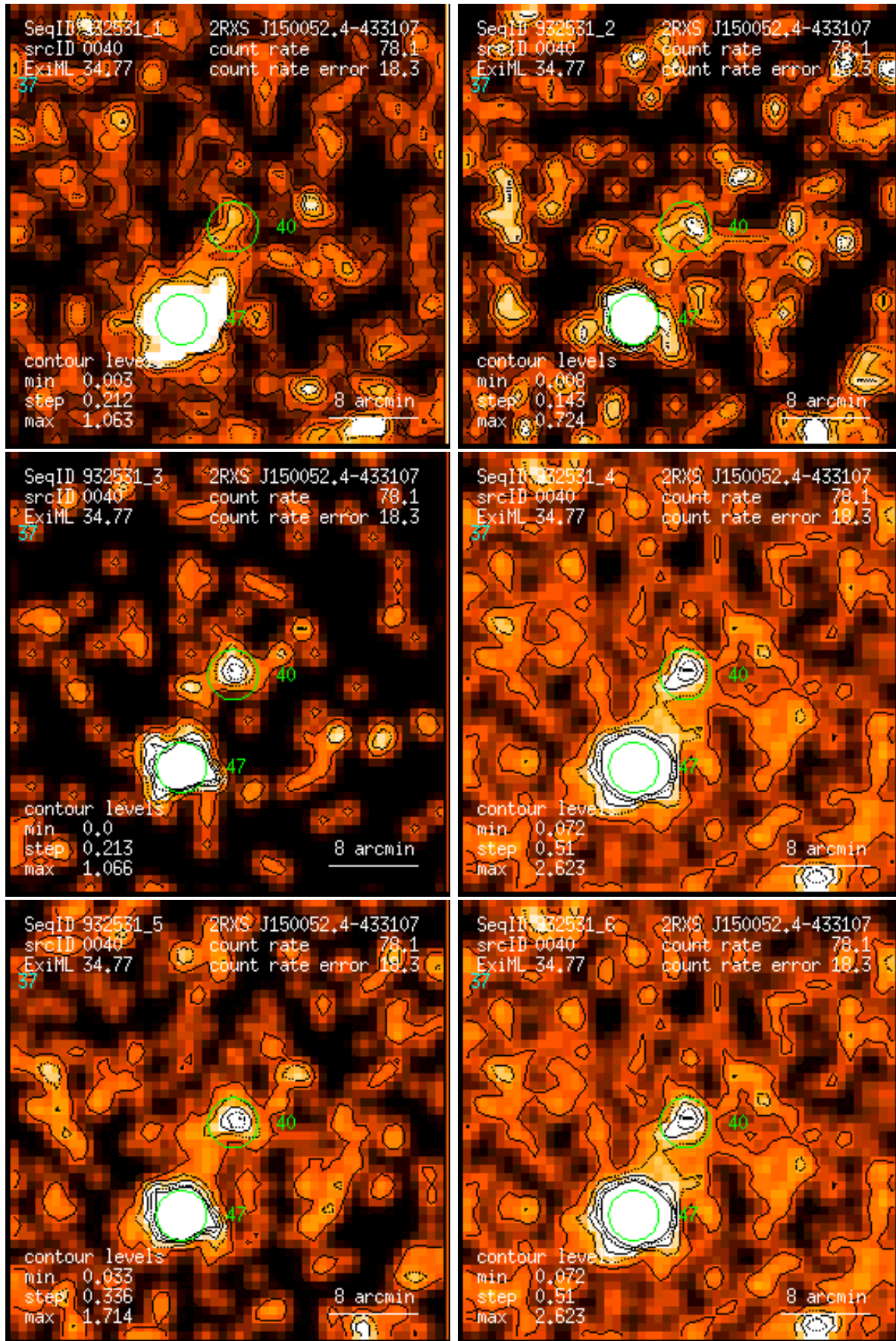
Figure 40: RASS 932531: detection 0040: band rate images, Gaussian filter: (1) PSPC channels 11 – 41, (2) 52 – 90, (3) 91 – 201, (4) 11 – 235, (5) 52 – 201, (6) 11 – 201. Broad band rates in counts/ks. Band rate contour levels in counts/ks/arcmin 2 .
