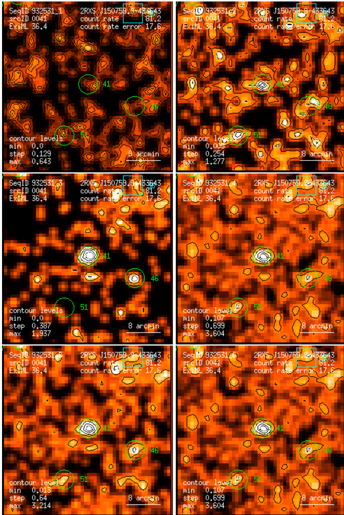
Figure 41: RASS 932531: detection 0041: band rate images, Gaussian filter: (1) PSPC channels 11 – 41, (2) 52 – 90, (3) 91 – 201, (4) 11 – 235, (5) 52 – 201, (6) 11 – 201. Broad band rates in counts/ks. Band rate contour levels in counts/ks/arcmin 2 .
