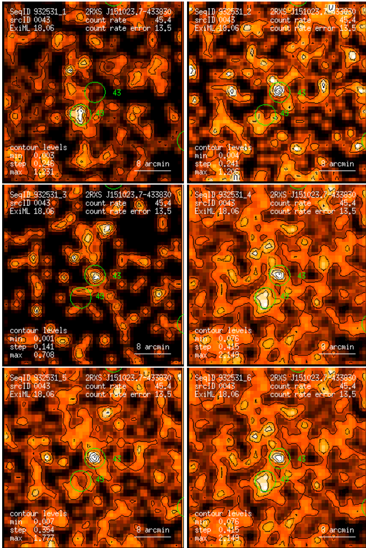
Figure 43: RASS 932531: detection 0043: band rate images, Gaussian filter: (1) PSPC channels 11 – 41, (2) 52 – 90, (3) 91 – 201, (4) 11 – 235, (5) 52 – 201, (6) 11 – 201. Broad band rates in counts/ks. Band rate contour levels in counts/ks/arcmin 2 .
