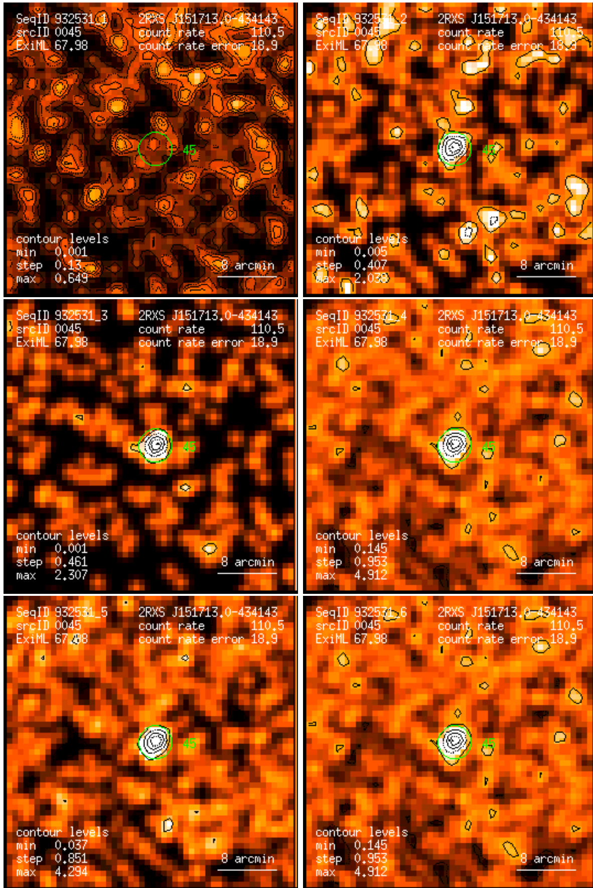
Figure 45: RASS 932531: detection 0045: band rate images, Gaussian filter: (1) PSPC channels 11 – 41, (2) 52 – 90, (3) 91 – 201, (4) 11 – 235, (5) 52 – 201, (6) 11 – 201. Broad band rates in counts/ks. Band rate contour levels in counts/ks/arcmin 2 .
