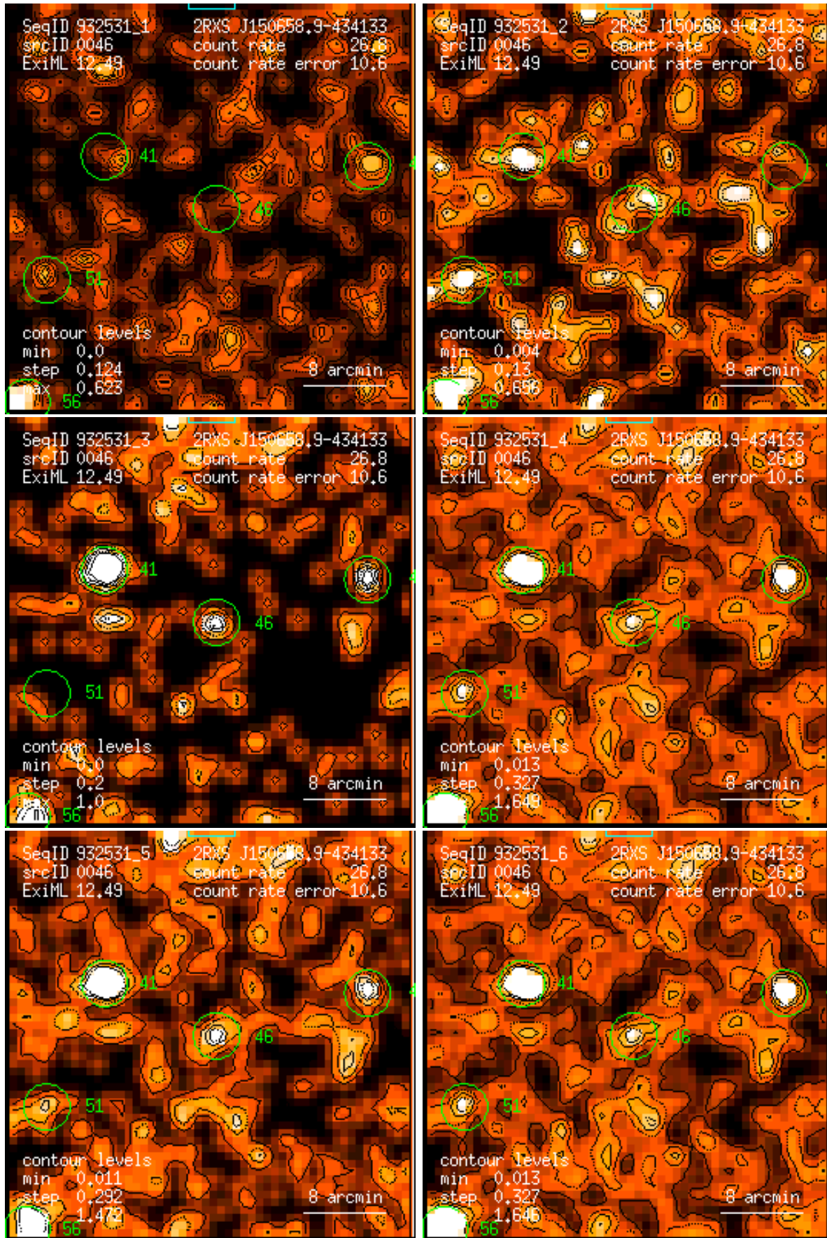
Figure 46: RASS 932531: detection 0046: band rate images, Gaussian filter: (1) PSPC channels 11 – 41, (2) 52 – 90, (3) 91 – 201, (4) 11 – 235, (5) 52 – 201, (6) 11 – 201. Broad band rates in counts/ks. Band rate contour levels in counts/ks/arcmin 2 .
