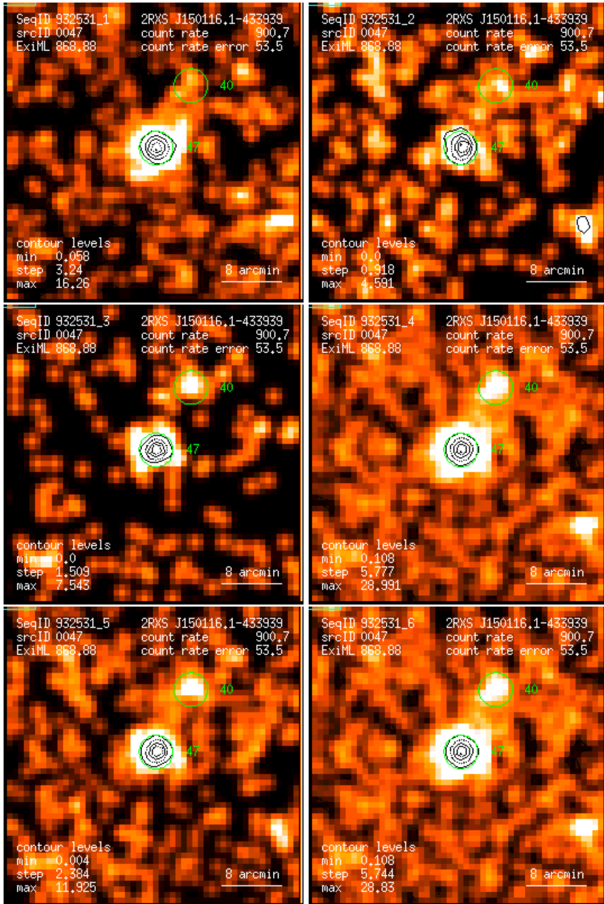
Figure 47: RASS 932531: detection 0047: band rate images, Gaussian filter: (1) PSPC channels 11 – 41, (2) 52 – 90, (3) 91 – 201, (4) 11 – 235, (5) 52 – 201, (6) 11 – 201. Broad band rates in counts/ks. Band rate contour levels in counts/ks/arcmin 2 .
