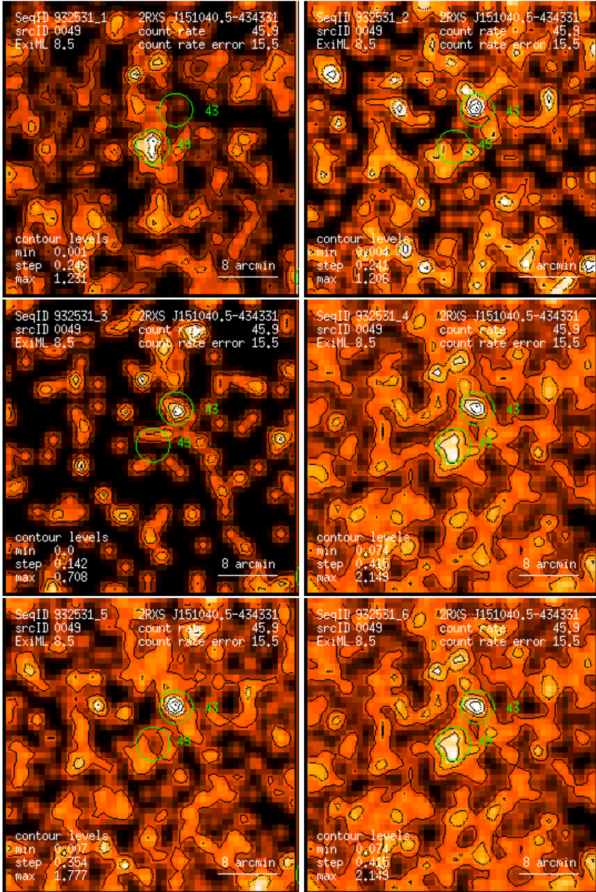
Figure 49: RASS 932531: detection 0049: band rate images, Gaussian filter: (1) PSPC channels 11 – 41, (2) 52 – 90, (3) 91 – 201, (4) 11 – 235, (5) 52 – 201, (6) 11 – 201. Broad band rates in counts/ks. Band rate contour levels in counts/ks/arcmin 2 .
