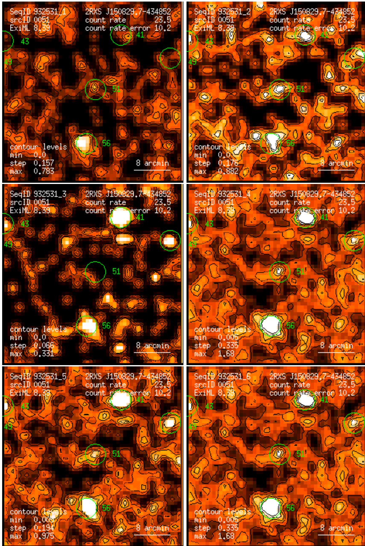
Figure 51: RASS 932531: detection 0051: band rate images, Gaussian filter: (1) PSPC channels 11 – 41, (2) 52 – 90, (3) 91 – 201, (4) 11 – 235, (5) 52 – 201, (6) 11 – 201. Broad band rates in counts/ks. Band rate contour levels in counts/ks/arcmin 2 .
