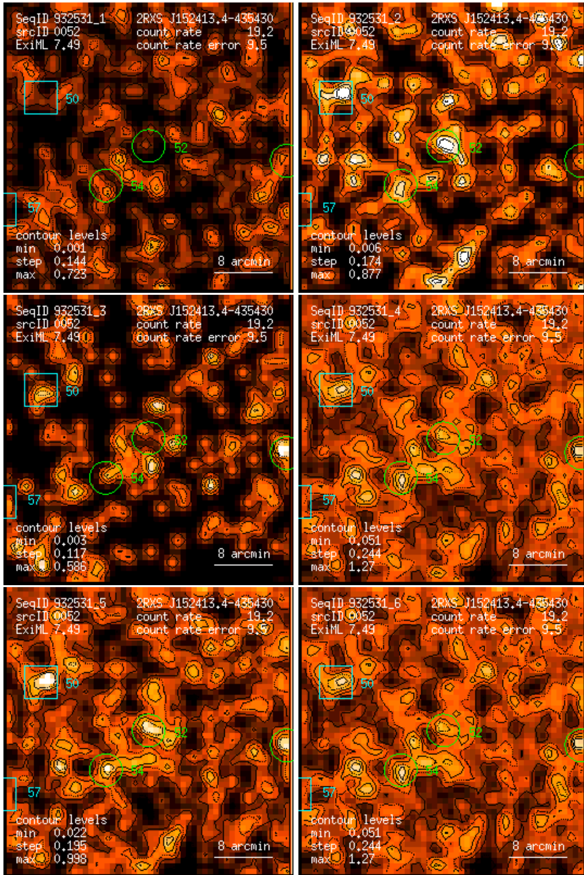
Figure 52: RASS 932531: detection 0052: band rate images, Gaussian filter: (1) PSPC channels 11 – 41, (2) 52 – 90, (3) 91 – 201, (4) 11 – 235, (5) 52 – 201, (6) 11 – 201. Broad band rates in counts/ks. Band rate contour levels in counts/ks/arcmin 2 .
