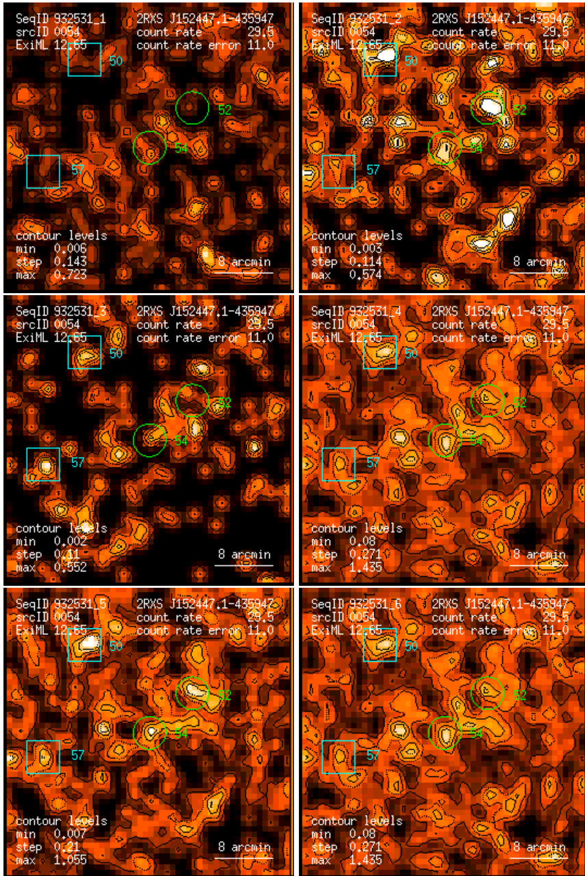
Figure 54: RASS 932531: detection 0054: band rate images, Gaussian filter: (1) PSPC channels 11 – 41, (2) 52 – 90, (3) 91 – 201, (4) 11 – 235, (5) 52 – 201, (6) 11 – 201. Broad band rates in counts/ks. Band rate contour levels in counts/ks/arcmin 2 .
