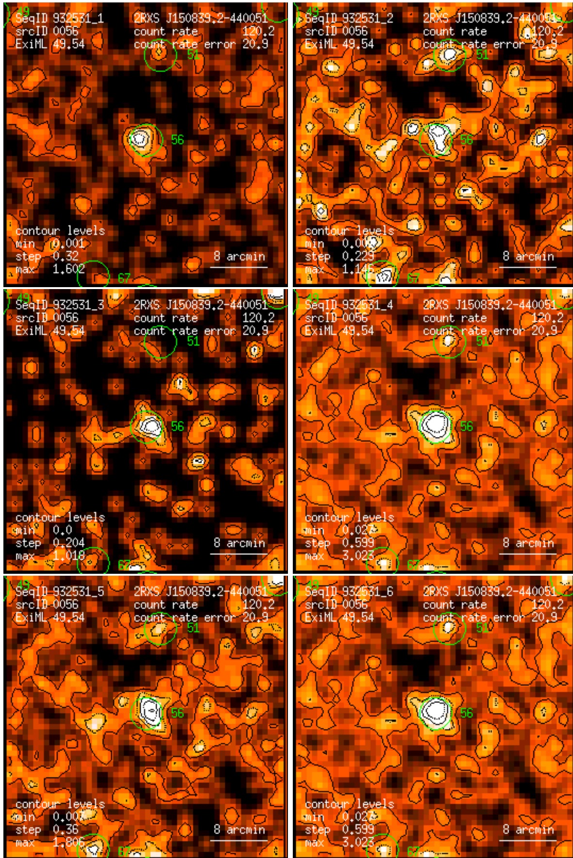
Figure 56: RASS 932531: detection 0056: band rate images, Gaussian filter: (1) PSPC channels 11 – 41, (2) 52 – 90, (3) 91 – 201, (4) 11 – 235, (5) 52 – 201, (6) 11 – 201. Broad band rates in counts/ks. Band rate contour levels in counts/ks/arcmin 2 .
