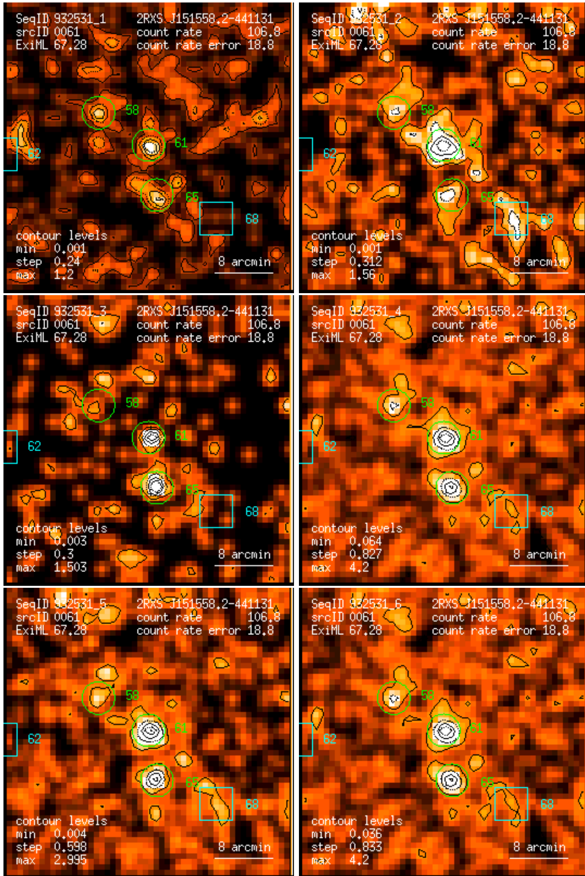
Figure 61: RASS 932531: detection 0061: band rate images, Gaussian filter: (1) PSPC channels 11 – 41, (2) 52 – 90, (3) 91 – 201, (4) 11 – 235, (5) 52 – 201, (6) 11 – 201. Broad band rates in counts/ks. Band rate contour levels in counts/ks/arcmin 2 .
