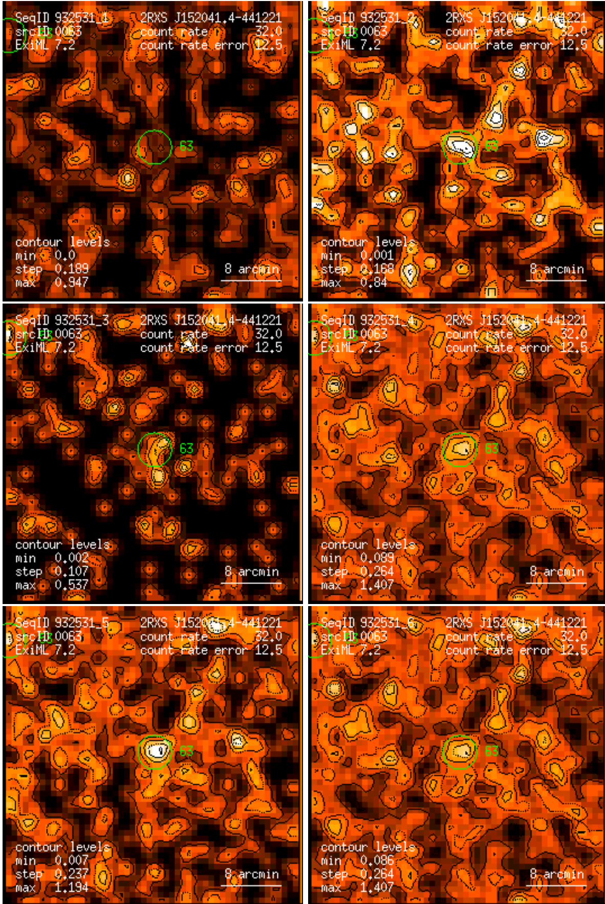
Figure 63: RASS 932531: detection 0063: band rate images, Gaussian filter: (1) PSPC channels 11 – 41, (2) 52 – 90, (3) 91 – 201, (4) 11 – 235, (5) 52 – 201, (6) 11 – 201. Broad band rates in counts/ks. Band rate contour levels in counts/ks/arcmin 2 .
