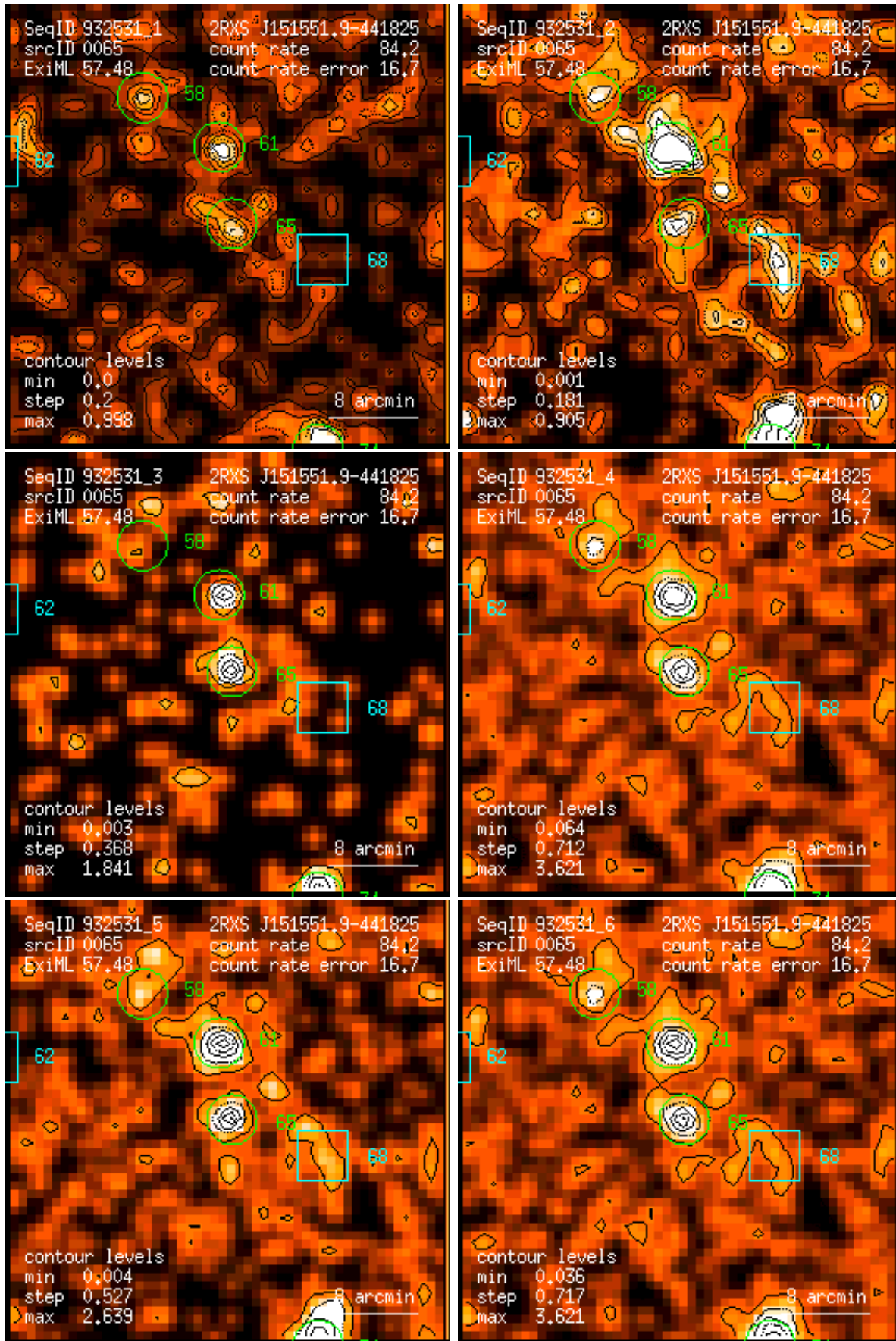
Figure 65: RASS 932531: detection 0065: band rate images, Gaussian filter: (1) PSPC channels 11 – 41, (2) 52 – 90, (3) 91 – 201, (4) 11 – 235, (5) 52 – 201, (6) 11 – 201. Broad band rates in counts/ks. Band rate contour levels in counts/ks/arcmin 2 .
