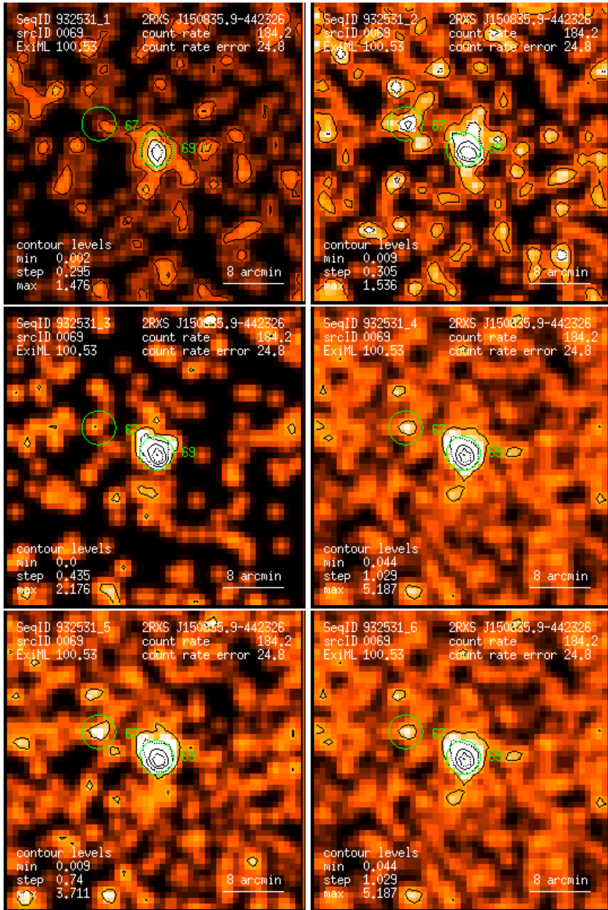
Figure 69: RASS 932531: detection 0069: band rate images, Gaussian filter: (1) PSPC channels 11 – 41, (2) 52 – 90, (3) 91 – 201, (4) 11 – 235, (5) 52 – 201, (6) 11 – 201. Broad band rates in counts/ks. Band rate contour levels in counts/ks/arcmin 2 .
