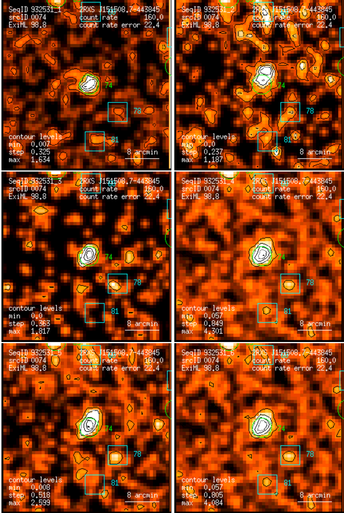
Figure 74: RASS 932531: detection 0074: band rate images, Gaussian filter: (1) PSPC channels 11 – 41, (2) 52 – 90, (3) 91 – 201, (4) 11 – 235, (5) 52 – 201, (6) 11 – 201. Broad band rates in counts/ks. Band rate contour levels in counts/ks/arcmin 2 .
