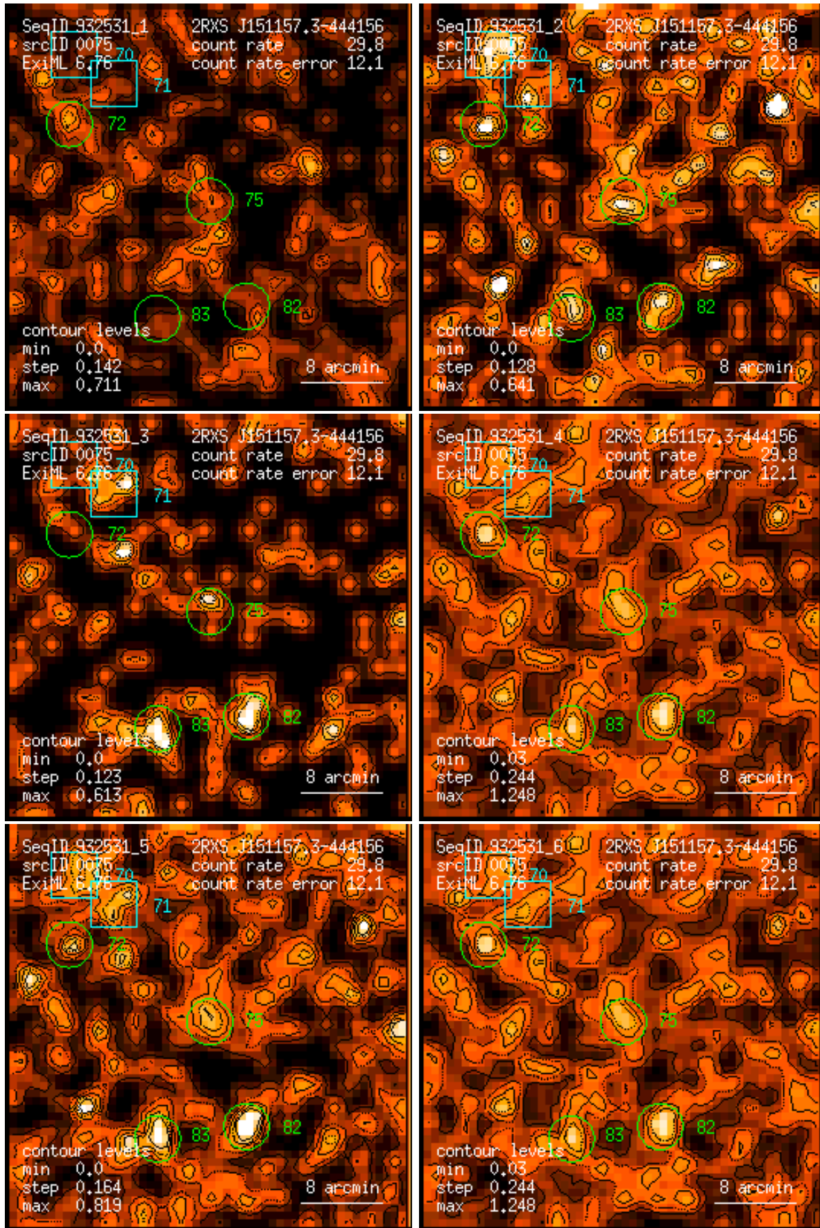
Figure 75: RASS 932531: detection 0075: band rate images, Gaussian filter: (1) PSPC channels 11 – 41, (2) 52 – 90, (3) 91 – 201, (4) 11 – 235, (5) 52 – 201, (6) 11 – 201. Broad band rates in counts/ks. Band rate contour levels in counts/ks/arcmin 2 .
