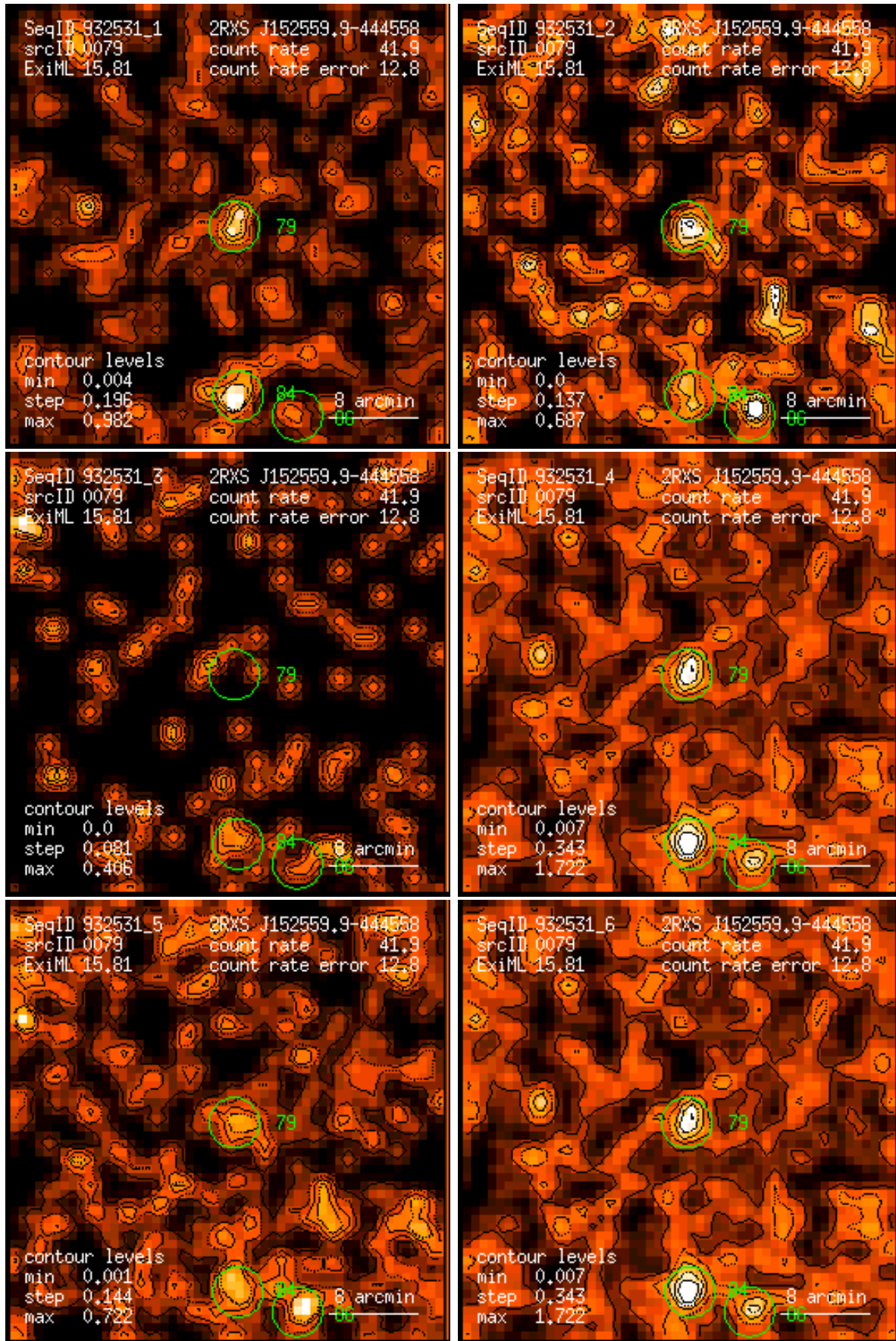
Figure 79: RASS 932531: detection 0079: band rate images, Gaussian filter: (1) PSPC channels 11 – 41, (2) 52 – 90, (3) 91 – 201, (4) 11 – 235, (5) 52 – 201, (6) 11 – 201. Broad band rates in counts/ks. Band rate contour levels in counts/ks/arcmin 2 .
