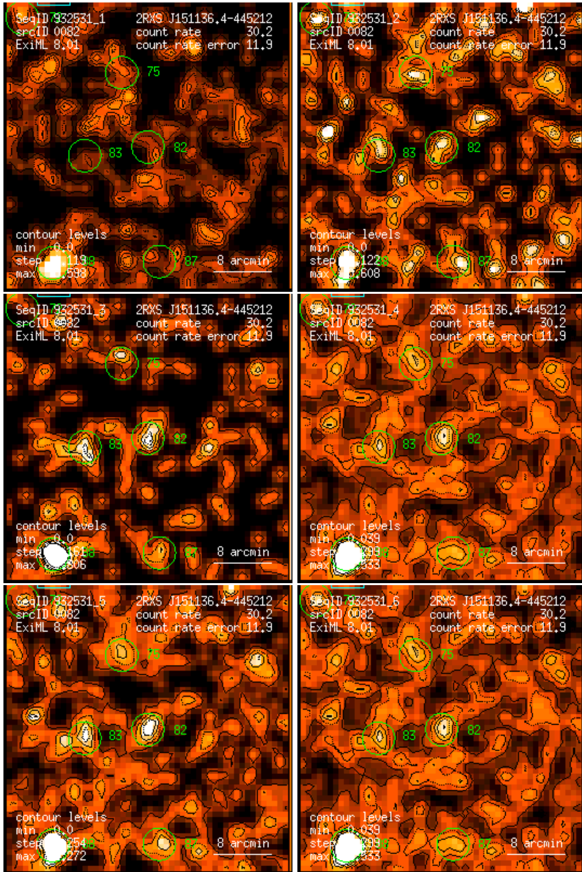
Figure 82: RASS 932531: detection 0082: band rate images, Gaussian filter: (1) PSPC channels 11 – 41, (2) 52 – 90, (3) 91 – 201, (4) 11 – 235, (5) 52 – 201, (6) 11 – 201. Broad band rates in counts/ks. Band rate contour levels in counts/ks/arcmin 2 .
