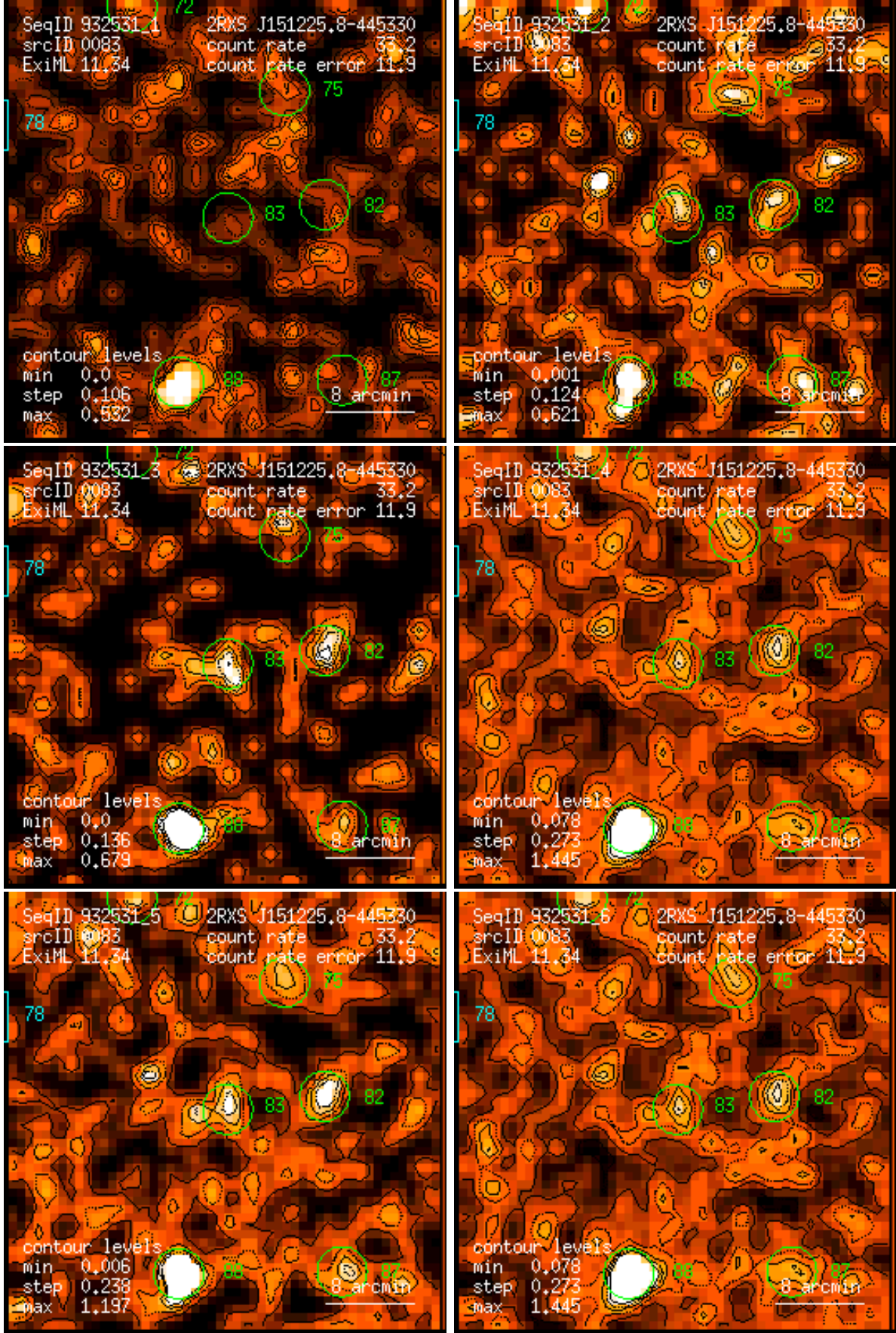
Figure 83: RASS 932531: detection 0083: band rate images, Gaussian filter: (1) PSPC channels 11 – 41, (2) 52 – 90, (3) 91 – 201, (4) 11 – 235, (5) 52 – 201, (6) 11 – 201. Broad band rates in counts/ks. Band rate contour levels in counts/ks/arcmin 2 .
