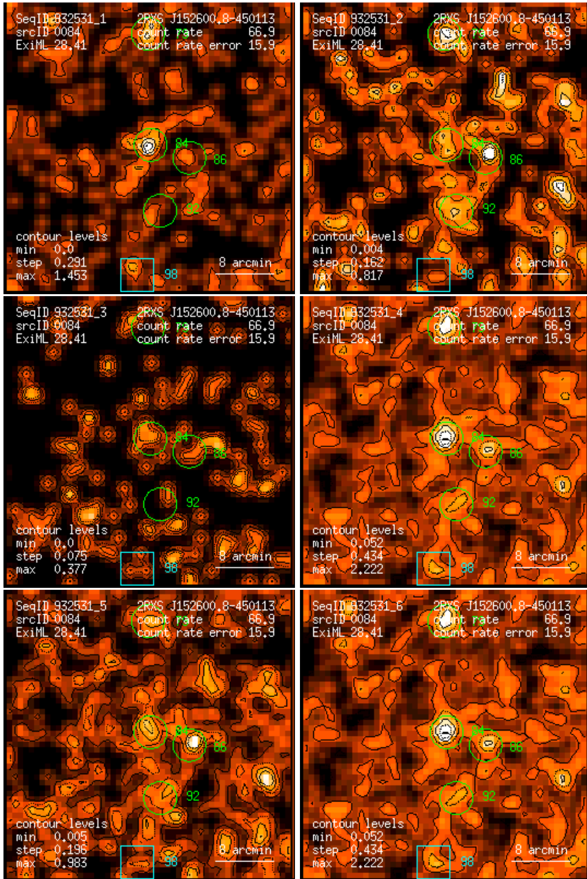
Figure 84: RASS 932531: detection 0084: band rate images, Gaussian filter: (1) PSPC channels 11 – 41, (2) 52 – 90, (3) 91 – 201, (4) 11 – 235, (5) 52 – 201, (6) 11 – 201. Broad band rates in counts/ks. Band rate contour levels in counts/ks/arcmin 2 .
