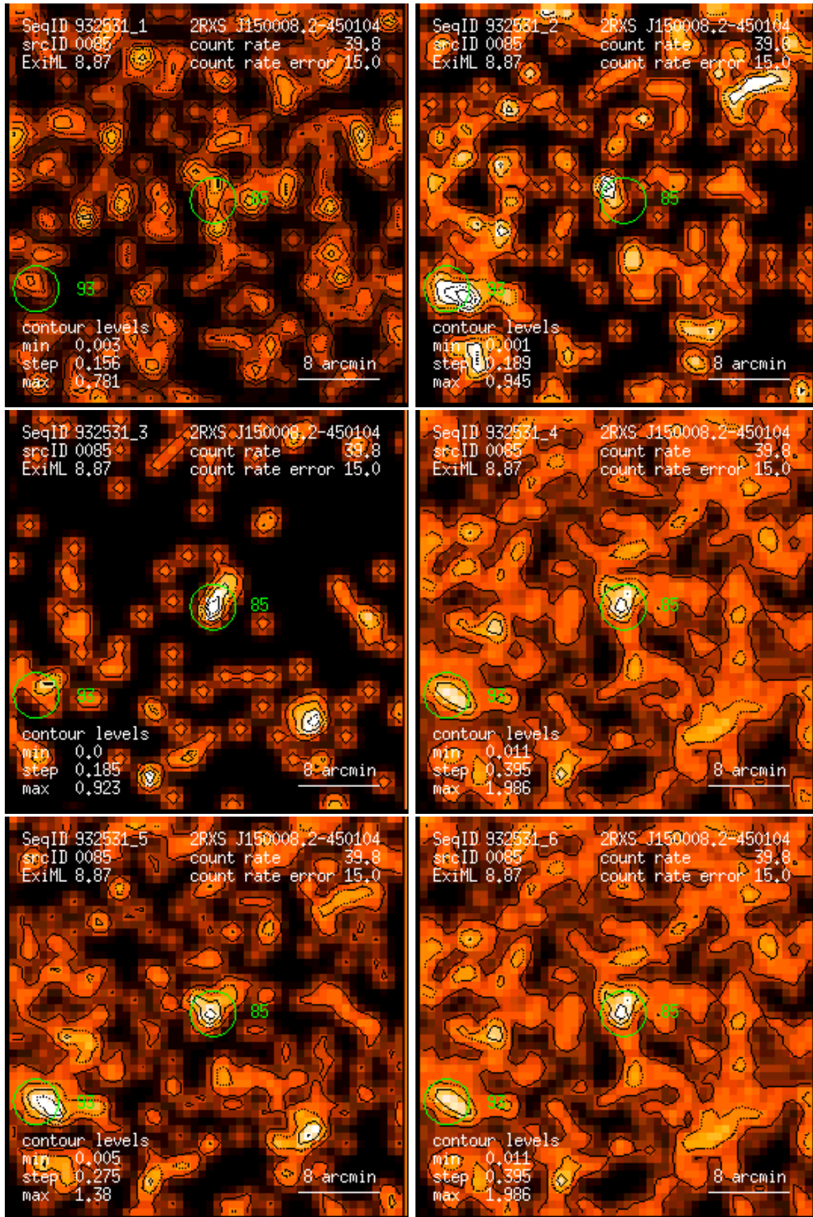
Figure 85: RASS 932531: detection 0085: band rate images, Gaussian filter: (1) PSPC channels 11 – 41, (2) 52 – 90, (3) 91 – 201, (4) 11 – 235, (5) 52 – 201, (6) 11 – 201. Broad band rates in counts/ks. Band rate contour levels in counts/ks/arcmin 2 .
